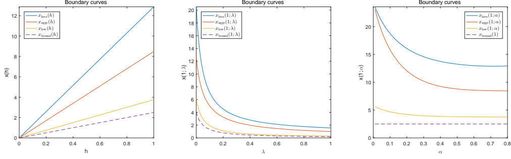
Figure 2: Boundary curves x_{\text{bound}} , x_{\text{low}} , x_{\text{aggr}} and x_{\text{lav}} with respect to the reference variable h (left), the force of mortality \lambda (middle), and the shortfall aversion parameter \alpha (right), respectively.
