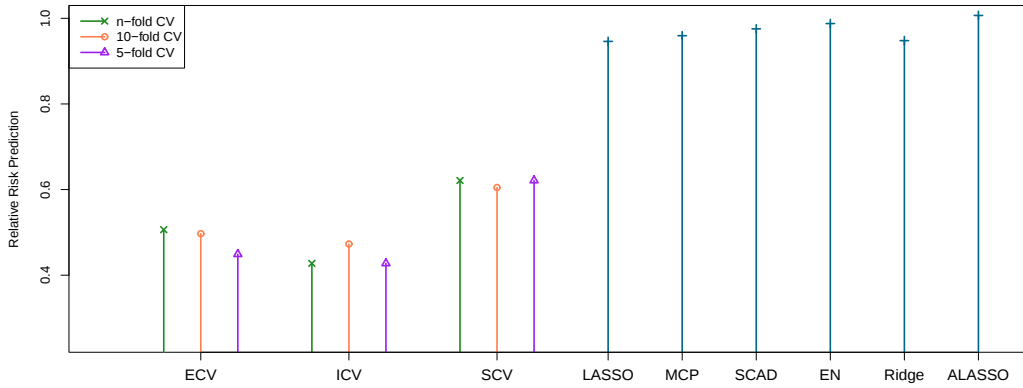
Figure 3: Prediction of the relative risk for a patient with column-wise medians of gene expressions in the mantle cell lymphoma study using the proposed methods with the first 100 convergence pathes under the greedy model averaging algorithms, and various regularization methods.
