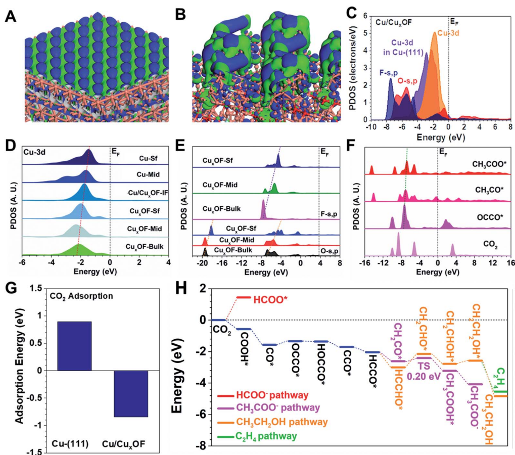
Fig. 4 The 3D contour plot for electronic distributions of (A) Cu-(111) and (B) Cu/Cu x OF. (C) PDOS of Cu/Cu x OF. Site-dependent PDOS of (D) Cu-3d, and (E) O-s,p and F-s,p in Cu/Cu x OF. (F) The PDOS of key adsorbates during the CO 2 RR process. (G) The comparison of CO 2 adsorption on Cu-(111) and Cu/Cu x OF. (H) The CO 2 RR reaction pathways on Cu/Cu x OF. The orange, red, and cyan balls in (A) and (B) represent Cu, O and F atoms, respectively, and the blue and green isosurfaces indicate the bonding and anti-bonding orbitals, respectively. The dashed lines in (D) and (E) represent the higher position of the band centers for Cu and O-s,p, and F-s,p, respectively.
