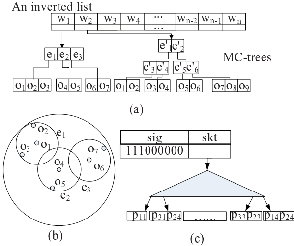
Fig. 3. IMC-tree illustration
