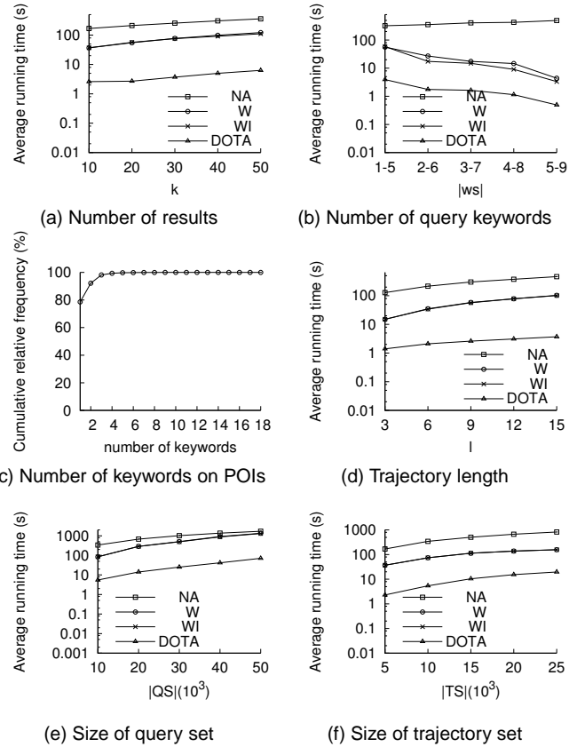
Fig. 6. Algorithm Efficiency
