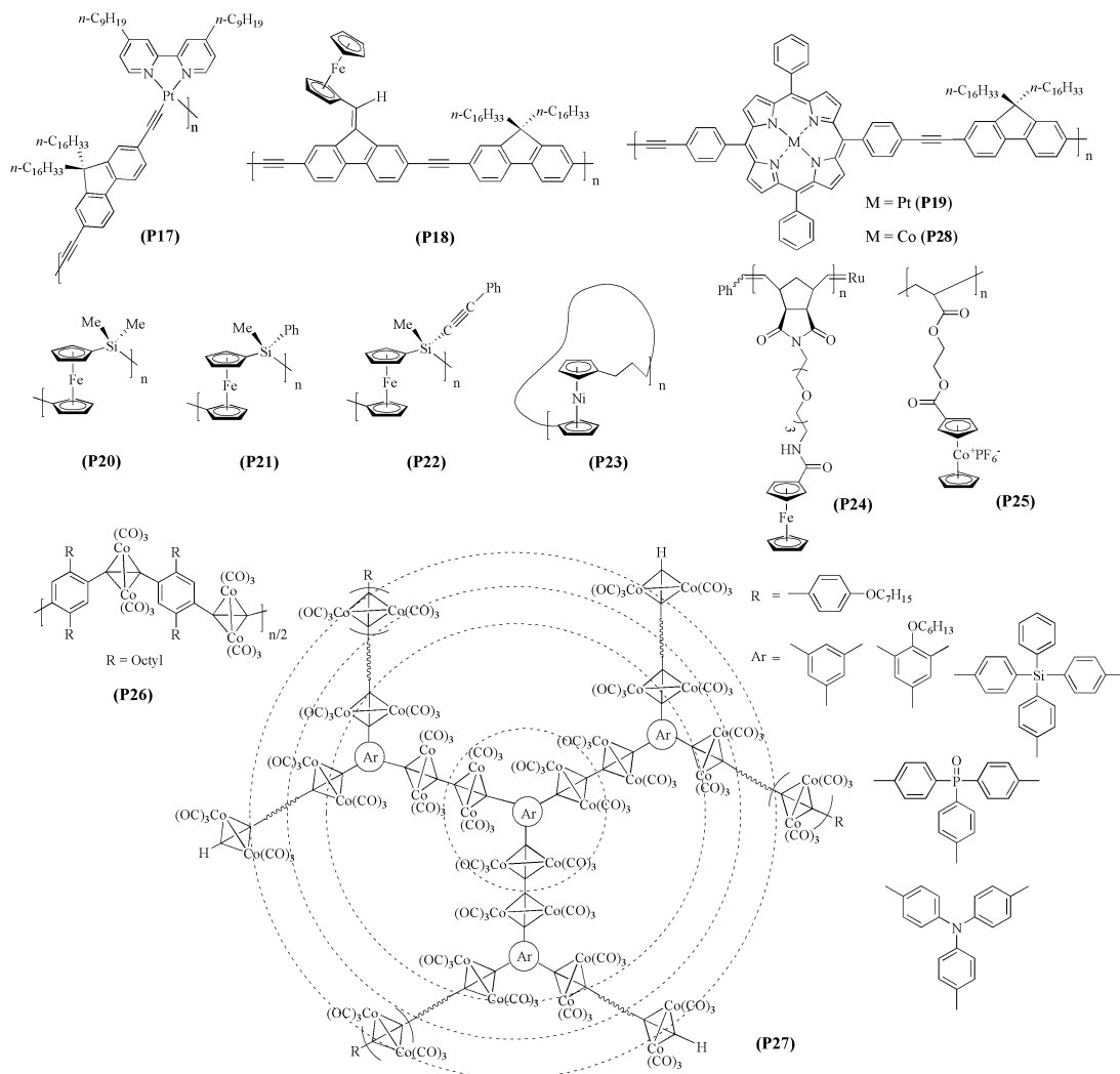
Fig. 4 Chemical structures of mononuclear metallopolymer precursors.
