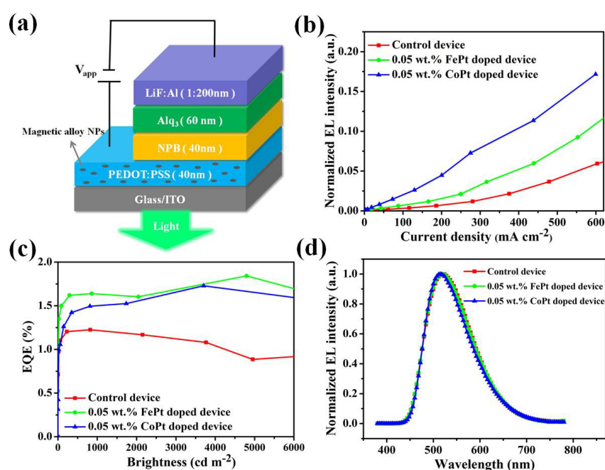
Fig. 19 (a) Schematic drawing illustrating the device structure of OLEDs with a PEDOT:PSS/magnetic NPs hybrid HTL, (b) relative EL intensity versus current density, (c) EQE versus brightness, and (d) normalized EL intensity versus wavelength.
