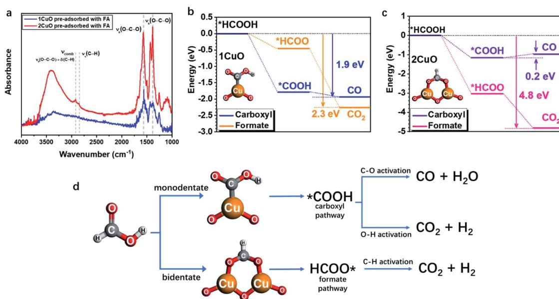
Fig. 6 (a) FTIR spectra of 1CuO and 2CuO with pre-adsorbed FA. The overall reaction energy trends of (b) 1CuO and (c) 2CuO . (d) The proposed reaction pathways of FA reforming, showing the interplay between adsorption configuration and pathway selection. 24,25,51
