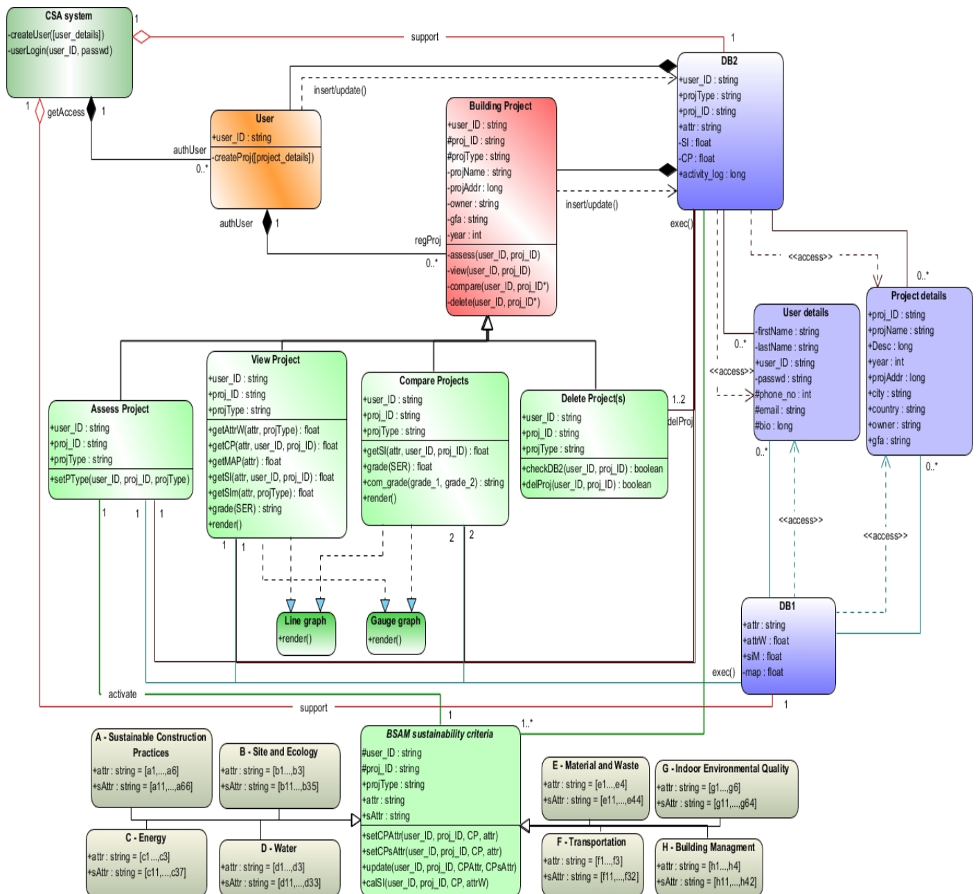
Figure 3: Class diagram for the proposed CSA system
