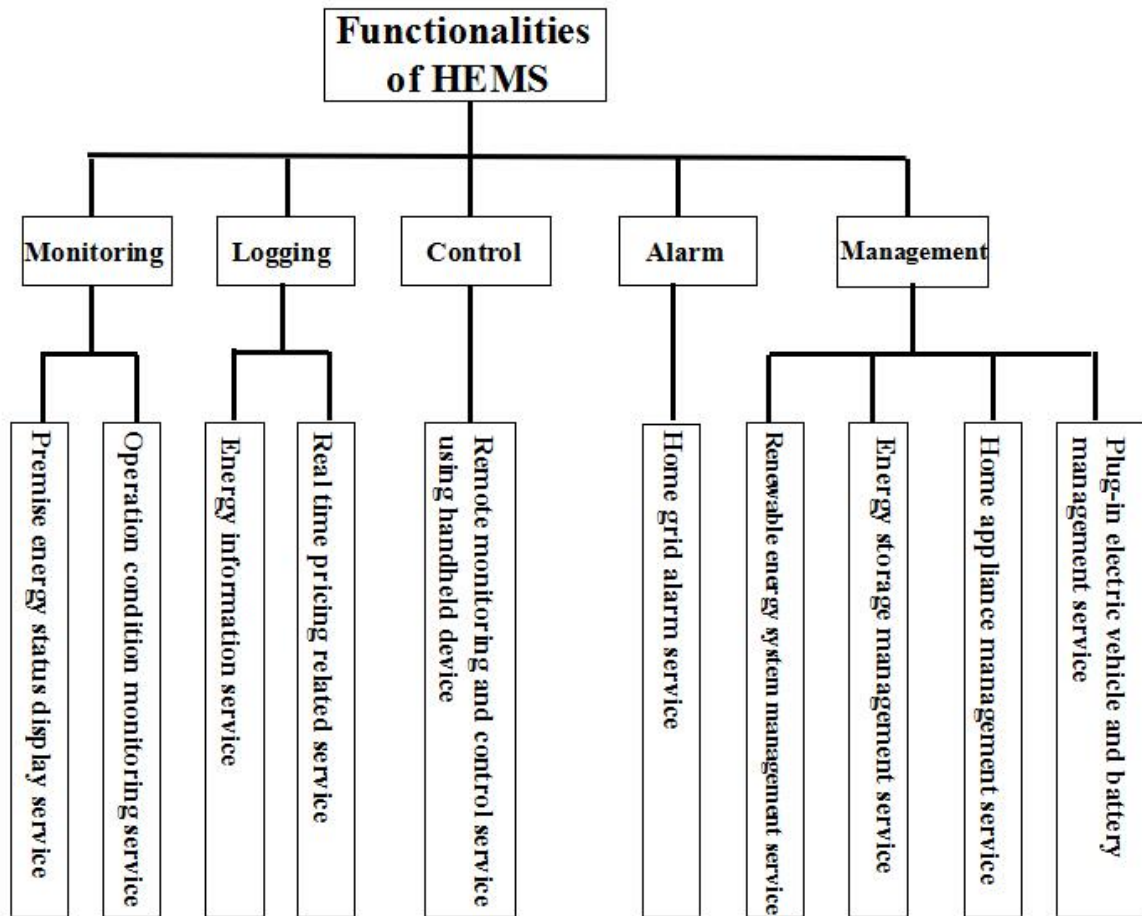
Figure 2 Functionalities of a representative smart HEMS
