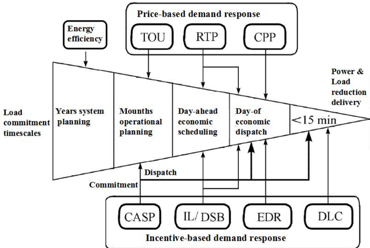
Figure 4 Demand response scheduling strategies in smart HEMS
