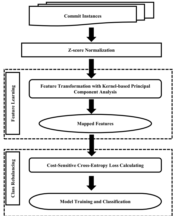
FIGURE 1 The overview of our KPIDL Framework
