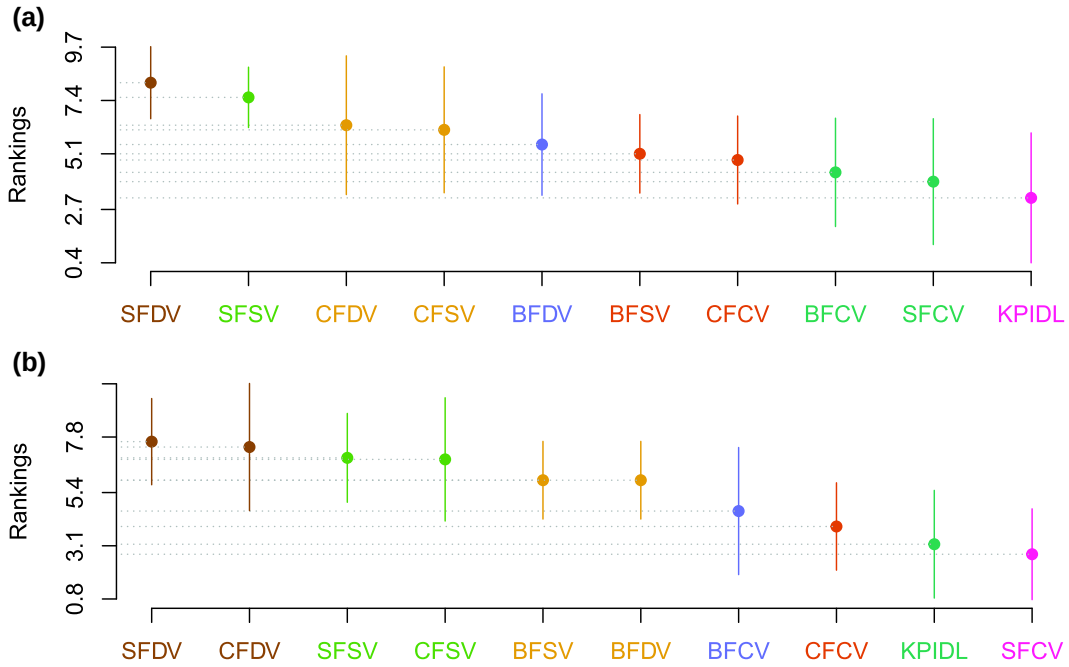
FIGURE 7 Scott-Knott Effect Size Difference (SKESD) test for our KPIDL method and cost-sensitive-based methods. (a) EAREcall, (b) EAF-measure
