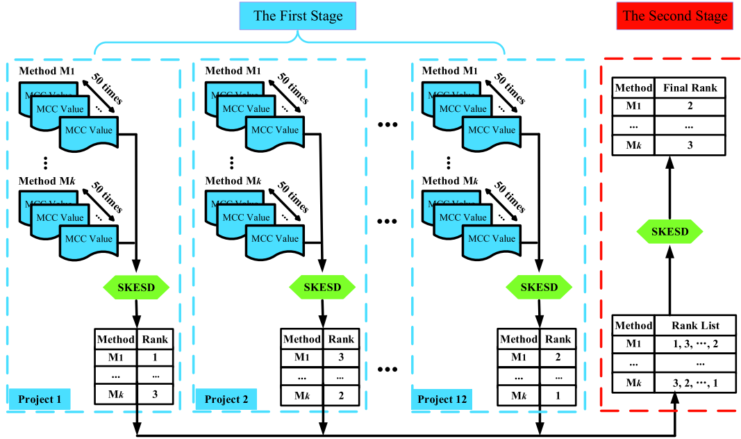
FIGURE 3 The operational process of Scott-Knott Effect Size Difference (SKESD) test
