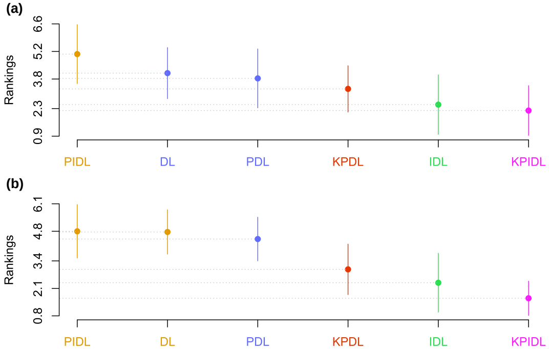
FIGURE 4 Scott-Knott Effect Size Difference test for KPIDL method and its variants. (a) EAREcall, (b) EAF-measure
