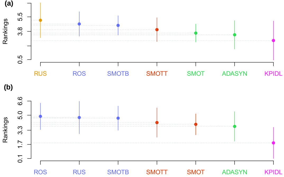
FIGURE 5 Scott-Knott Effect Size Difference test for our KPIDL method and sampling-based methods. (a) EAREcall, (b) EAF-measure
