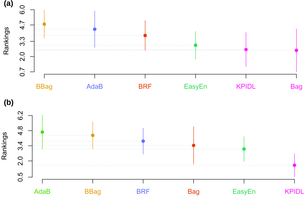
FIGURE 6 Scott-Knott Effect Size Difference test for our KPIDL method and ensemble-based methods. (a) EAREcall, (b) EAF-measure
