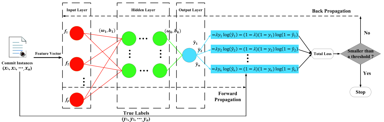
FIGURE 2 The iterative process of Deep Neural Network (DNN)
