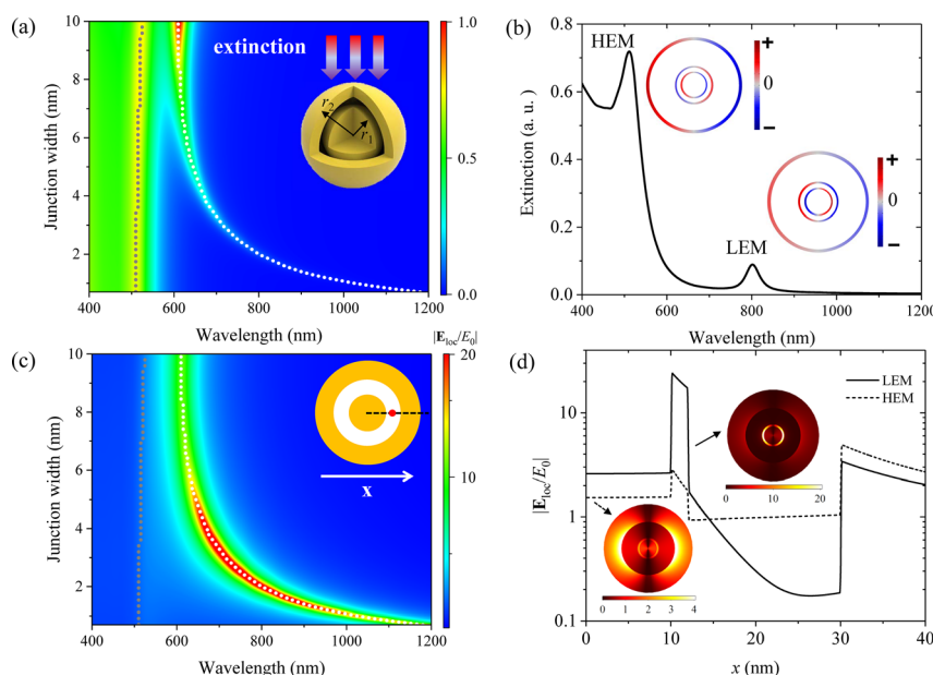
Figure 1: Linear optical responses of the gold core–molecule–shell (CMS) insulating junction as a function of the junction width varying from 0.7 to 10 nm.
