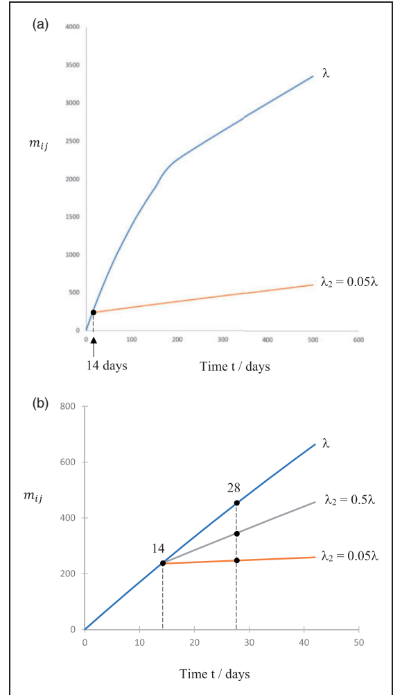
Figure 2. Number of infections at different rates. (a) Over a long time and (b) Over a shorter period.
