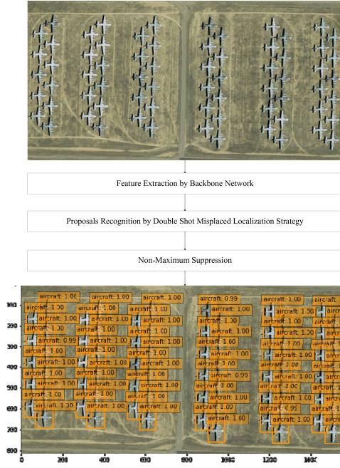
Fig. 1. Architecture of our proposed DNN.
