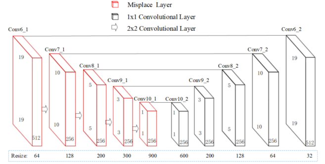
Fig. 2. Architecture of extra layers of our proposed DNN.
