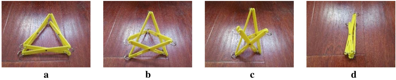
Figure 15. Motion sequence of spatial triangular polar scissor unit
