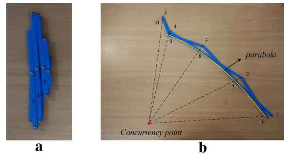
Figure 16. Planar polar scissor mechanism: a folded state, b deployment state
