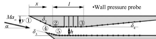
Fig. 1 Main dimensions of the model 32 ( \alpha = -10^\circ , \delta_2 = -21.5^\circ , \delta_3 = -9.5^\circ , \delta_4 = 5^\circ , h = 15 mm, see the origin reference for details).
