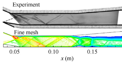
Fig. 4 Comparison of an experimental schlieren image and numerical Mach number contour for a specified back pressure ratio of 7.
