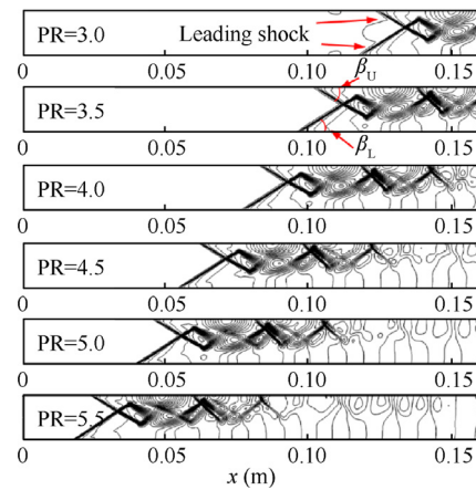
Fig. 6 Pressure contours under uniform incoming flow conditions ( Ma_1 = 2.5 , Re = 2.09 \times 10^7 \text{ m}^{-1} , PR = 3.0\text{--}5.5 ).
