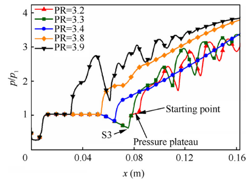
Fig. 21 Pressure distributions along lower wall in PR rising process under condition of background waves.
