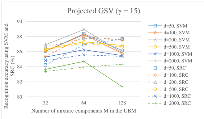
Fig. 11. Microphone recognition accuracy using projected GSV, with the relevance factor equal 15.
