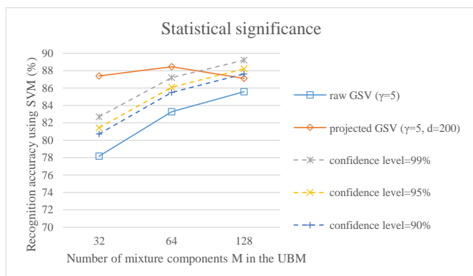
Fig. 14. Statistical significance of the performance improvement offered by the projection method employing SVM as the classifier.
