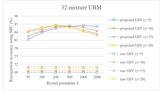
Fig. 6. Microphone recognition accuracy employing SRC as the classifier, with the GSV adapted from a 32-mixture UBM.
