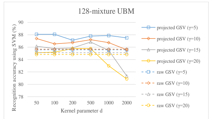
Fig. 5. Microphone recognition accuracy employing SVM as the classifier, with the GSV adapted from a 128-mixture UBM.
