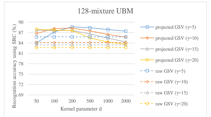
Fig. 8. Microphone recognition accuracy employing SRC as the classifier, with the GSV adapted from a 128-mixture UBM.
