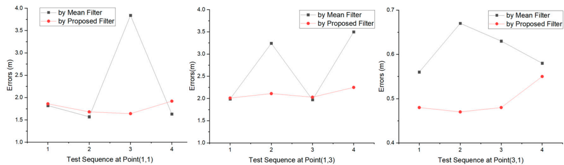
Figure 8. Positioning error comparison with the proposed filter and the mean filter at point (1,1), point (1,3) and point (3,1).
