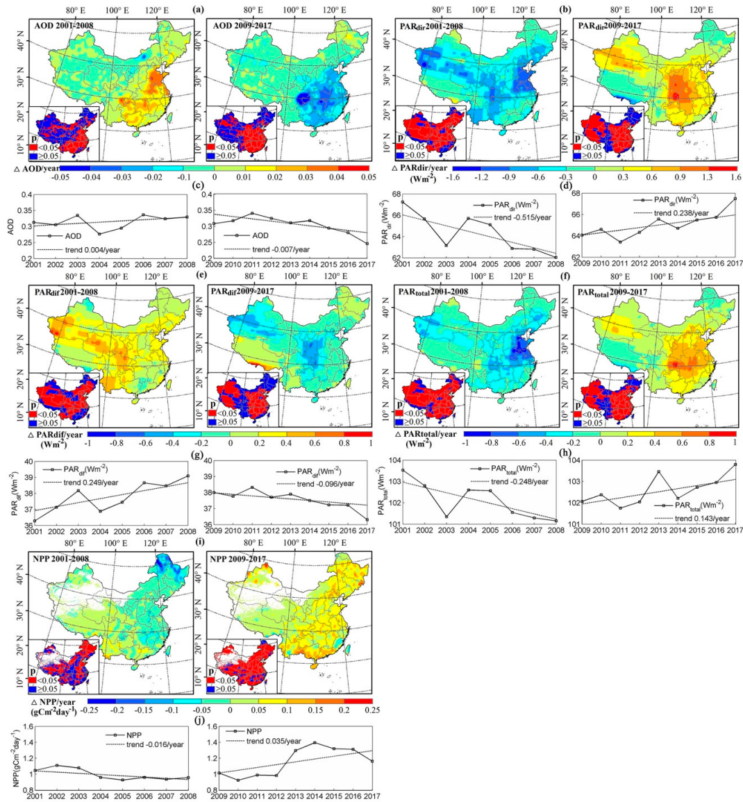
Figure 5. Spatial variation of trends for AOD (a), \text{PAR}_{\text{dir}} (b), \text{PAR}_{\text{dif}} (e), \text{PAR}_{\text{total}} (f) and NPP (i) during 2001–2008 and 2009–2017. Red area indicates trends with p -value < 0.05 and blue area indicates trends with p -value \geq 0.05 . The temporal variation of annual mean values over China are (c,d,g,h,j).
