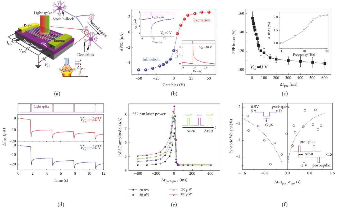
FIGURE 9: (a) Schematics of graphene/CNT based ORRAM synaptic device. (b) STP: post-synaptic current stimulated with an optical pulse at various gate bias. (c) PPF index as a function of pulse interval. (d) LTP obtained by combining optical pulse and voltage pulse. (e) Illustration of STLR learning rule. (f) Illustration of STDP learning rule. Reproduced with permission from [54].
