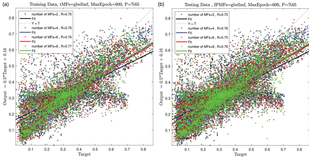
Figure 3. (a) Training with using two inputs and different number of MFs (ANFIS method). (b) Testing with using two inputs and different number of MFs (ANFIS method).
