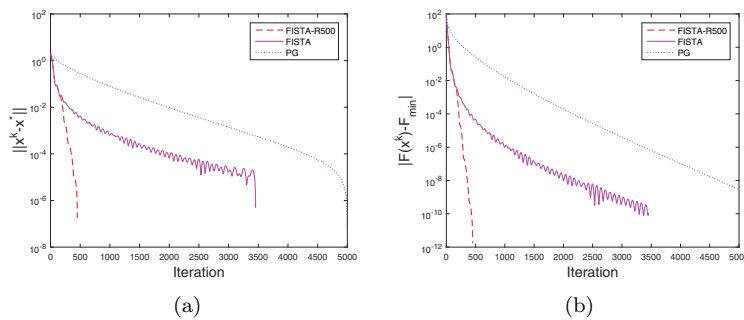
FIG. 2. l_1 -logistic: n = 5000, m = 500, s = 50 .
