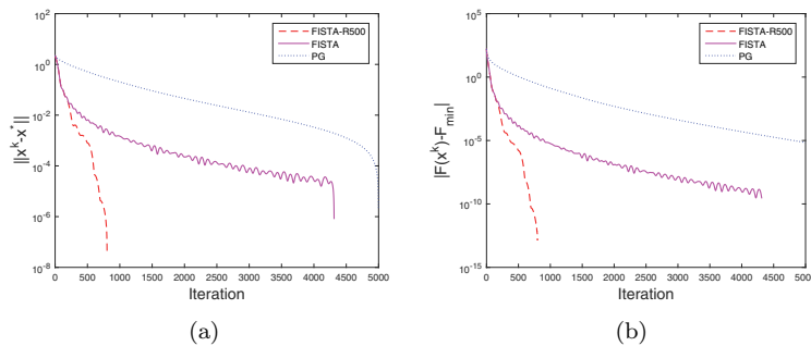
FIG. 3. l_1 -logistic: n = 8000, m = 800, s = 80 .
