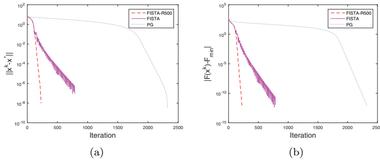
FIG. 4. l_1 - ls : n = 3000, m = 300, s = 30 .
