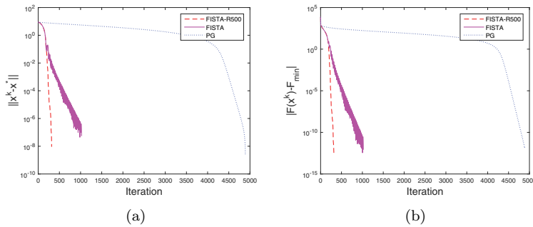
FIG. 6. l_1 - ls : n = 8000, m = 800, s = 80 .
