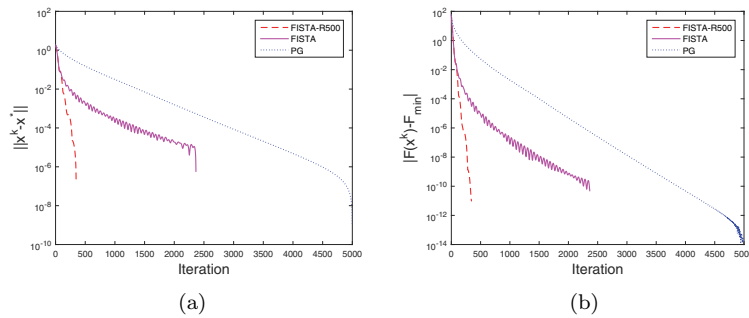
FIG. 1. l_1 -logistic: n = 3000, m = 300, s = 30 .
