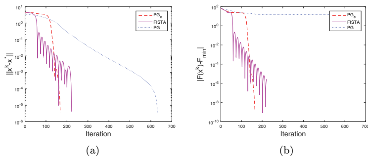
FIG. 7. Nonconvex quadratic problem.
