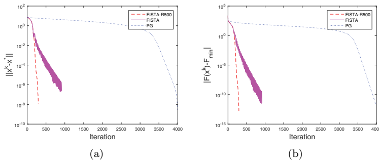
FIG. 5. l_1 - ls : n = 5000, m = 500, s = 50 .
