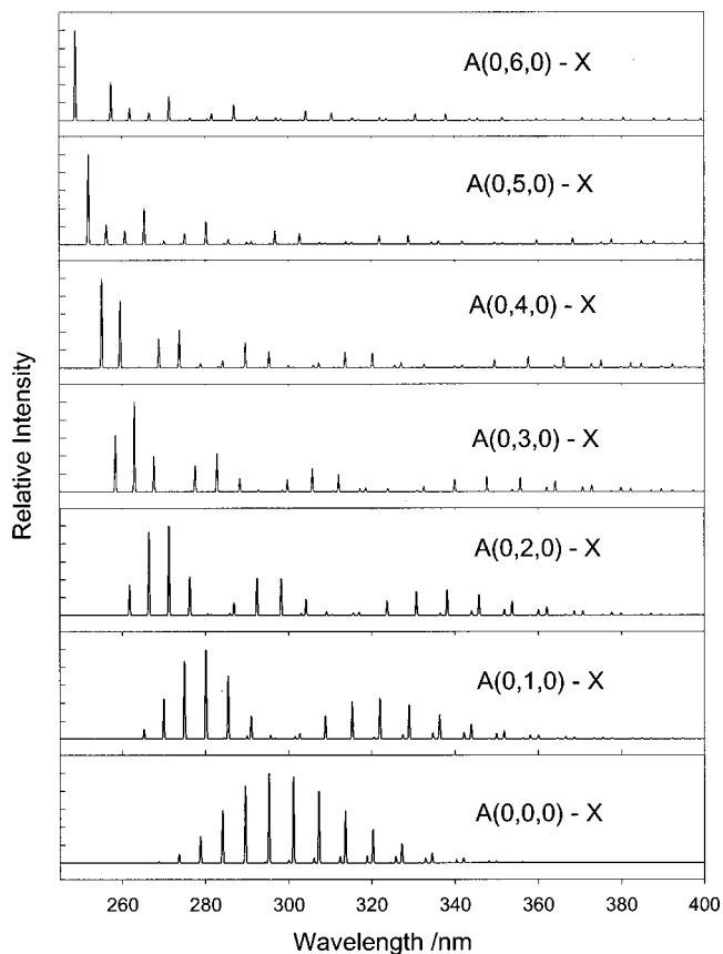
FIG. 4. Simulated spectra of the \tilde{A}^1B_1(0,v_2,0) \rightarrow \tilde{X}^1A_1 CF 2 single vibronic level (SVL) emissions, for v_2=0-6 , employing the CASSCF/MRCI/aug-cc-pVQZ(no g) and RCCSD(T)/aug-cc-pVQZ PEF for the two states, respectively, the experimental geometry from Ref. 4 for the \tilde{X}^1A_1 state and the IFCA geometry of r_e(\text{CF})=1.317 \text{ \AA} and \theta_e(\text{FCF})=121.25^\circ for the \tilde{A}^1B_1 state.
