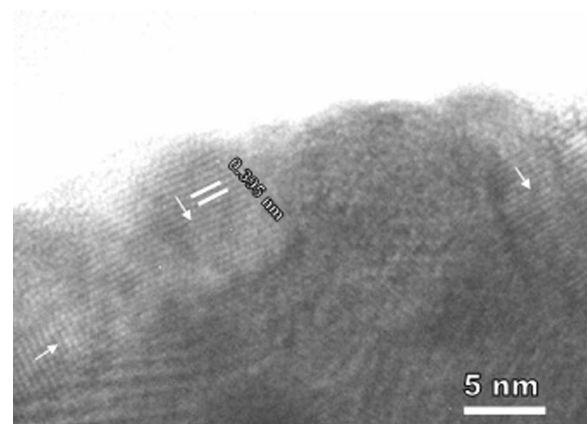
FIG. 3. HRTEM image of the BFO nanotubes, the arrows indicate the \{101\} atomic planes with lattice spacing around 0.395 nm.
