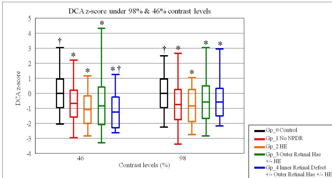
Fig. 3. Comparison of the DC amplitude z-scores (DCA z ) for Groups 0 to 4 at high (98%) and low (46%) contrast levels (* : p<0.05 when compared with Group 0; † : p<0.05 when compared with Group 1) (Box plot: centre line – the mean; the edges of the box – ± 1 standard deviation; the edges of the vertical bars – range)
