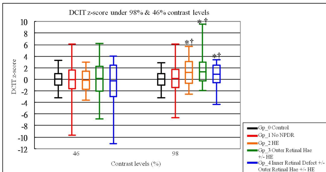
Fig. 5. Comparison of DC implicit time z-scores (DCIT_z) for Group 0 to 4 at high (98%) and low (46%) contrast levels (* : p < 0.05 when compared to Group 0; † :
