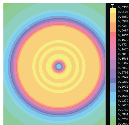
Fig. 11: Magnetic field distribution of the proposed induction cooker
