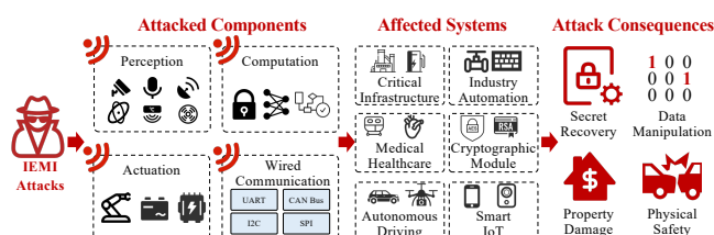
Figure 1: IEMI attacks affect cyber-physical systems by compromising the operation of perception, computation, actuation, and wired communication components, which are widely integrated into critical infrastructures, medical healthcare devices, smart IoT systems, etc., causing various consequences.
