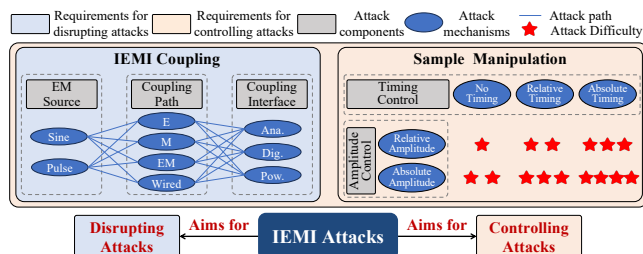
Figure 3: The essential components of IEMI disrupting and controlling attacks. By mapping attack objectives to the required knowledge and mechanisms, it's possible to compare the difficulty of executing different IEMI attacks.
