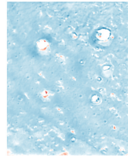
(c) 影像光度法DEM与摄影测量DEM差异图 (c) Difference map of photoclinometric DEM and photogrammetric DEM
