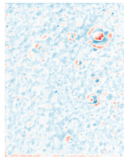
(e) 影像光度法DEM与LDEM差异图 (e) Difference map of photoclinometric DEM and LDEM
