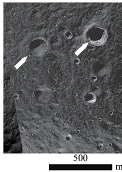
(a) 实验区2所有NAC光照像素拼接影像 (a) NAC image mosaic from all the illuminated pixels in study area 2
