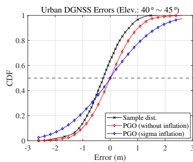
Fig. 12. The CDF of the PGO for urban DGNSS errors for elevation angles observed from 40° to 45°. Since the overbounding conditions cannot be satisfied, the sigma inflation is designed to stop early at the 50th iteration.
