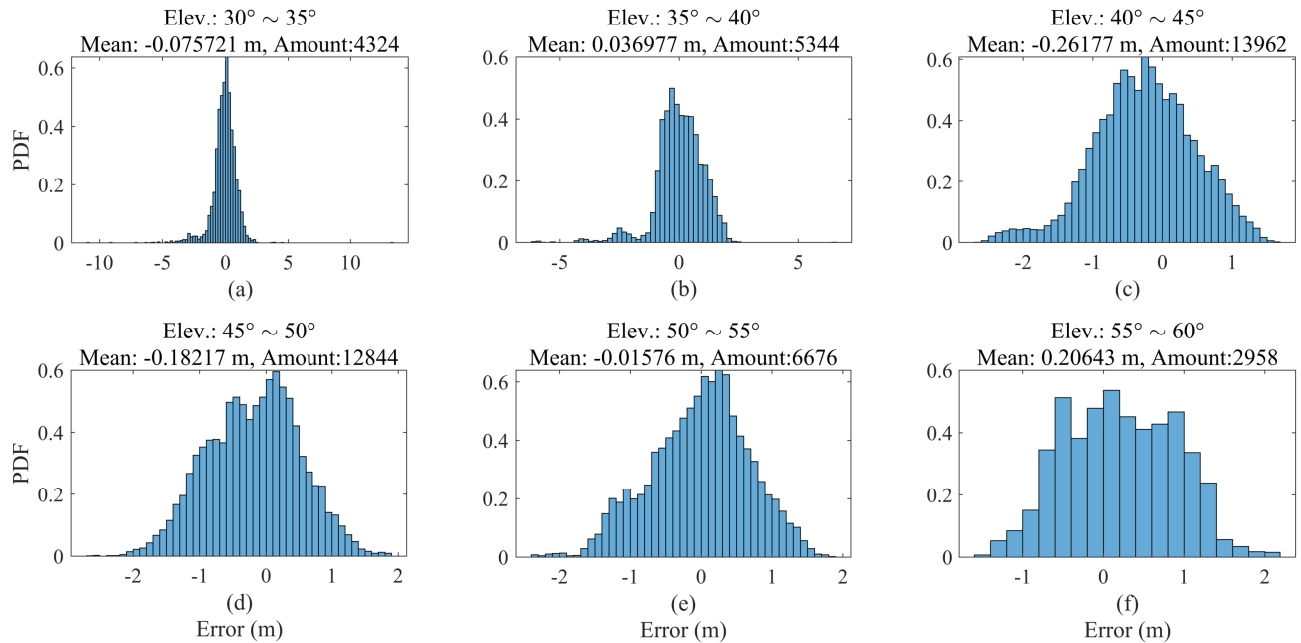
Fig. 14. The histogram of the urban DGNSS error with the SNR larger than 35 dB and the elevation angle larger than 30^\circ in each 5^\circ elevation angle bin. The mean value of the DGNSS error and the amount of samples in each bin are presented in the title of each subplot. The bins with less than 5 samples are not plotted.
