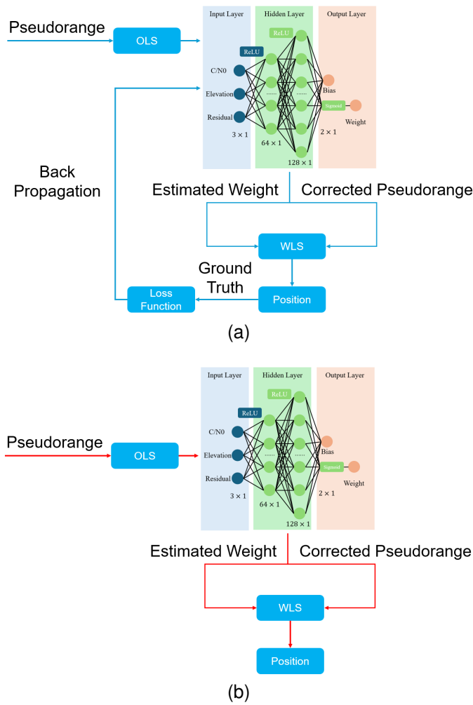
Fig. 2. The overview of our training and prediction process
