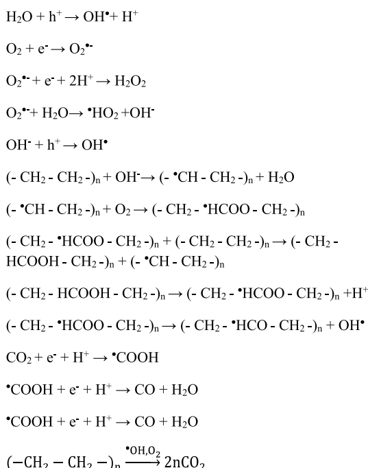
Scheme 1. Possible reactions during photocatalytic breakdown of PE.
