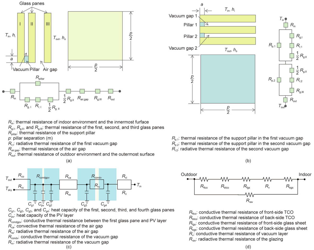
Fig. 8. The diagrams of the thermal resistance network of different vacuum glazing structures. (a) Hybrid vacuum glazing; (b) triple vacuum glazing; (c) laminated PV-vacuum glazing; (d) hollow PV-vacuum glazing. TCO: transparent conductive oxide. Reproduced from Refs. [16,91] with permission.
