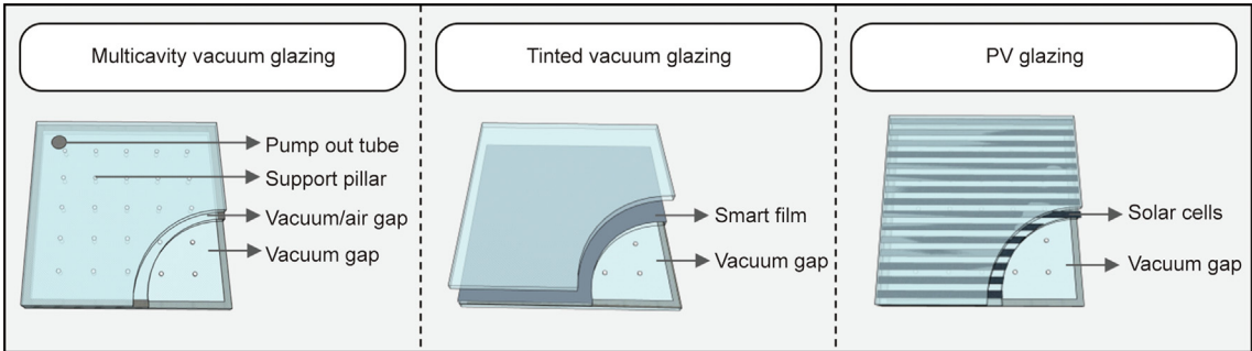
Fig. 6. Structure diagram of mainstream composite vacuum glazing.
