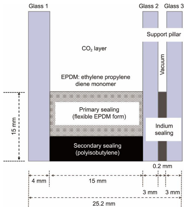
Fig. 14. Optimal design of hybrid vacuum glazing [119].
