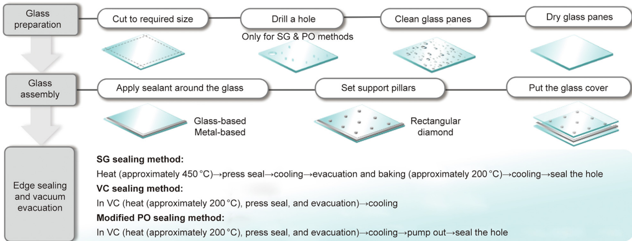
Fig. 4. Detailed steps of three vacuum glazing fabrication methods.
