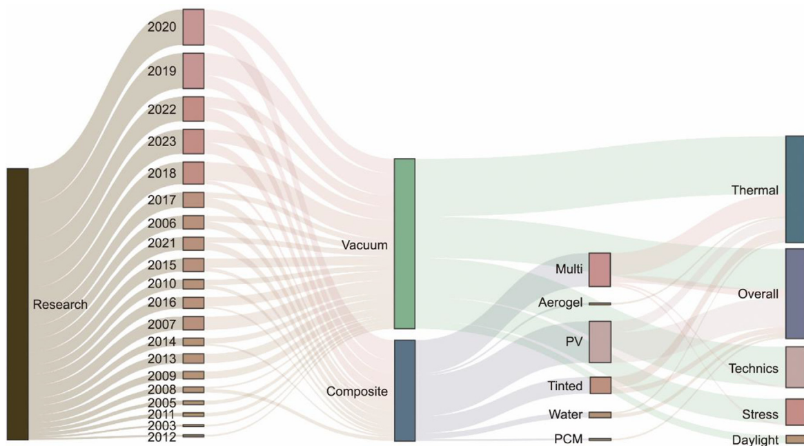
Fig. 3. Research objects and focused performance. “Vacuum” refers to conventional double-pane vacuum glazing, “Composite” refers to vacuum glazing composited with other technologies, like multi-pane vacuum glazing (Multi), aerogel-vacuum glazing (Aerogel), PV-vacuum glazing (PV), tinted-vacuum glazing (Tinted), water flow vacuum glazing (Water), and PCM-vacuum glazing (PCM). The performance studied include thermal performance (Thermal), overall performance (Overall), preparation techniques (Technics), stress performance (Stress) and daylight performance (Daylight).
