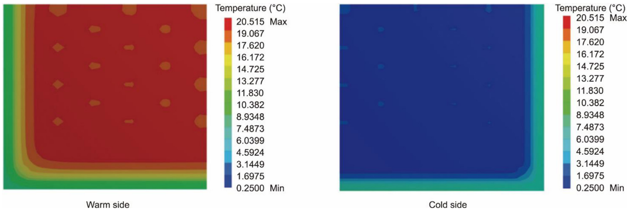
Fig. 10. Finite-element mesh of vacuum glazing (500 mm × 500 mm) and the temperature distribution on both warm and cold surfaces [94].
