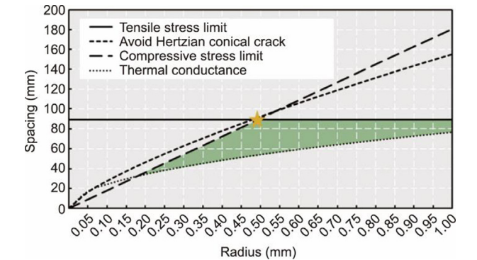
Fig. 5. Schematic diagram of the design for an array of support pillars. Reproduced from Ref. [45] with permission.
