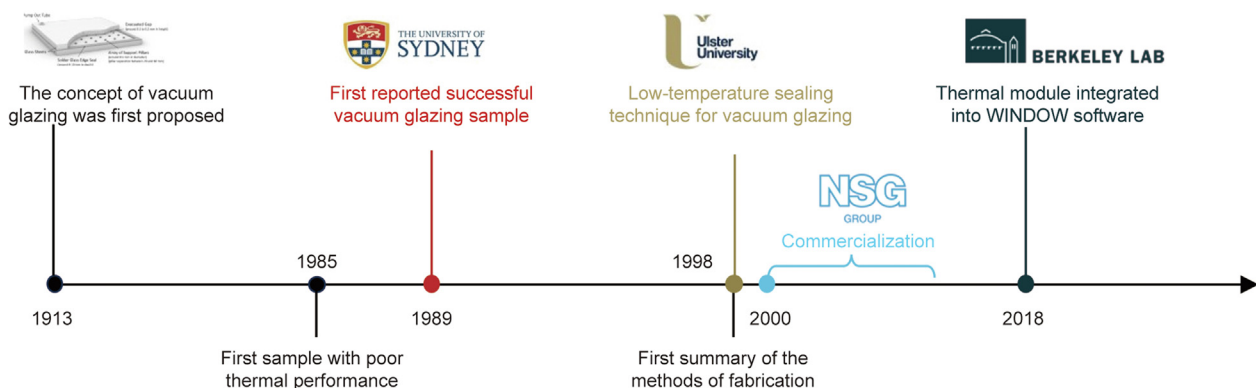
Fig. 1. Development history diagram of vacuum glazing.
