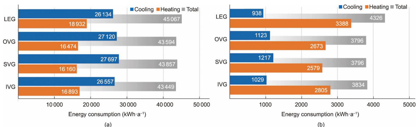
Fig. 17. Energy consumption with different glazing units in (a) office and (b) residential buildings [46].
