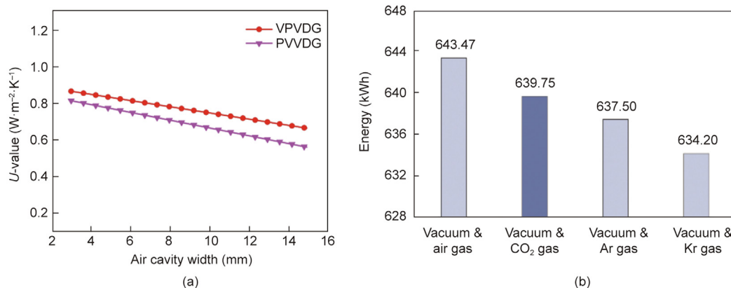
Fig. 16. (a) The impacts of insulating cavity thickness on the thermal performance. (b) The impact of insulating cavity types on the thermal performance. Reproduced from Refs. [97,119] with permission.
