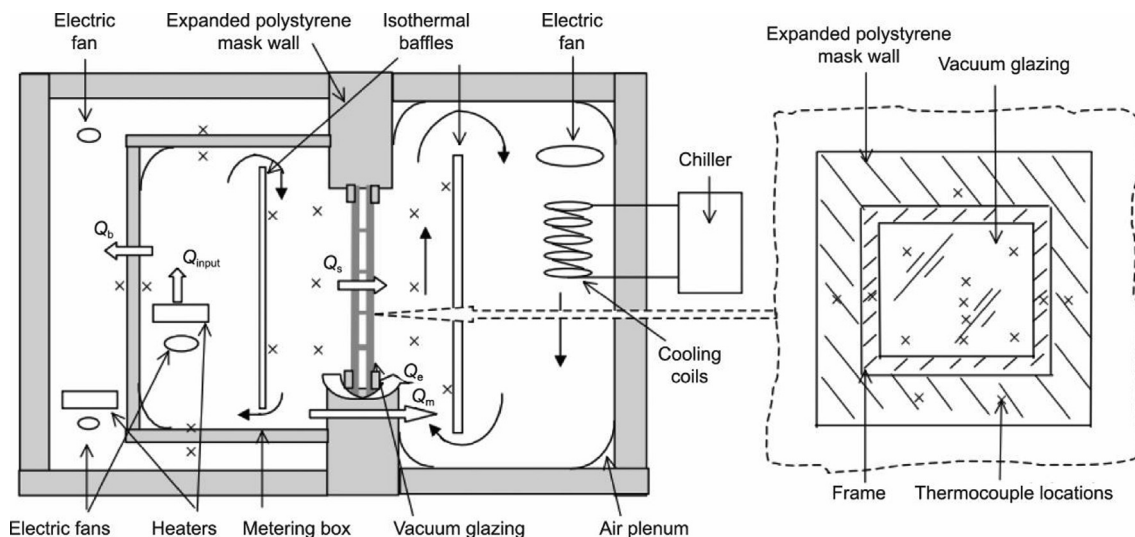
Fig. 12. Schematic diagram of the guarded hot box device. Reproduced from Ref. [95] with permission.
