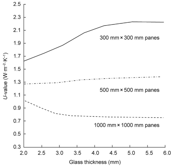
Fig. 11. The impacts of the glass thickness on U -value of vacuum glazing. Reproduced from Ref. [44] with permission.
