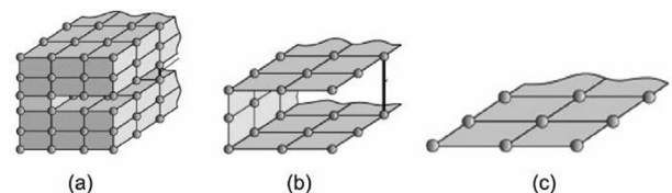
Fig. 9. (a) Solid element, (b) double shell-layer element, and (c) single shell-layer element. Reproduced from Ref. [93] with permission.
