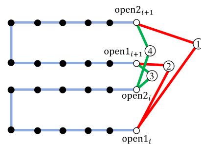
Figure 3. Illustration of all position connections between layer i and i + 1 . (1): open2_i is the entry node and the UAV will navigate to open1_i and open2_{i+1} accordingly, and exit at open1_{i+1} . (2): open2_i is the entry node and the UAV will navigate to open1_i and open1_{i+1} accordingly, and exit at open2_{i+1} . (3): open1_i is the entry node and the UAV will navigate to open2_i and open1_{i+1} accordingly, and exit at open2_{i+1} . (4): open1_i is the entry node and the UAV will navigate to open2_i and open2_{i+1} accordingly, and exit at open1_{i+1} .
