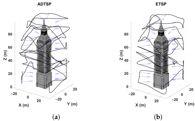
Figure 6. Simulated minimum snap trajectories. (a) Minimum snap trajectory for ADTSP. (b) Minimum snap trajectory for ETSP.
