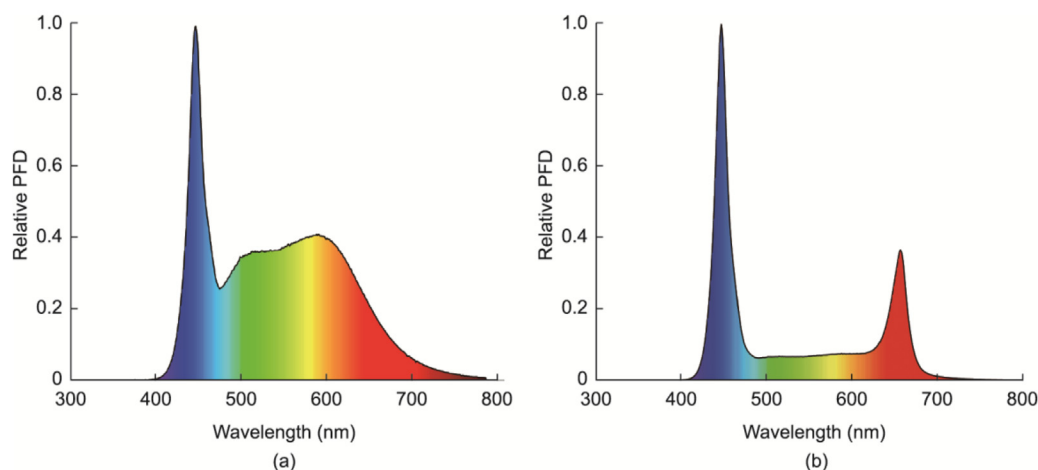
Fig. 1. Spectral composition of the LED light. (a) Spectral composition of white LED light; (b) spectral composition of white + blue + red LED light.
