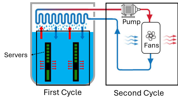
Figure A.1: A two-phase immersion cooling system
