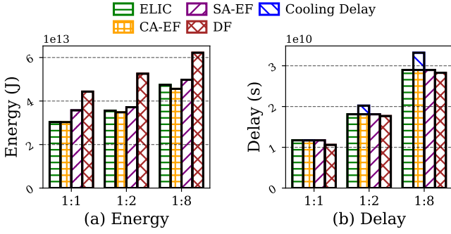
Figure G.1: Performance of GPU quantities with coolant FC-72 during pretraining
