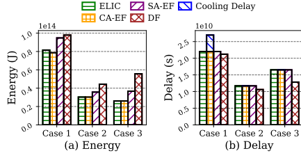
Figure 2: Performance of various cases with coolant FC-72 during pretraining.
