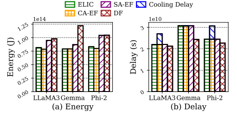
Figure 4: Performance of various training jobs on Case 1 and FC-72.
