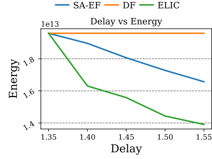
Figure G.2: Performance of Delay Requirements with coolant FC-72 during pretraining
