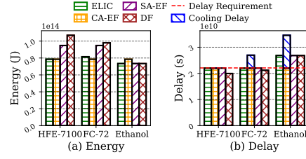
Figure 3: Performance of various coolants on Case 1 during pretraining.
