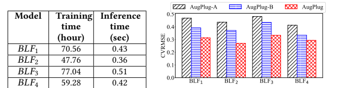
Figure 9: Comparison of AugPlug and the variants.
