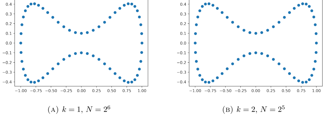
FIGURE 1. Initial nodal distribution.
