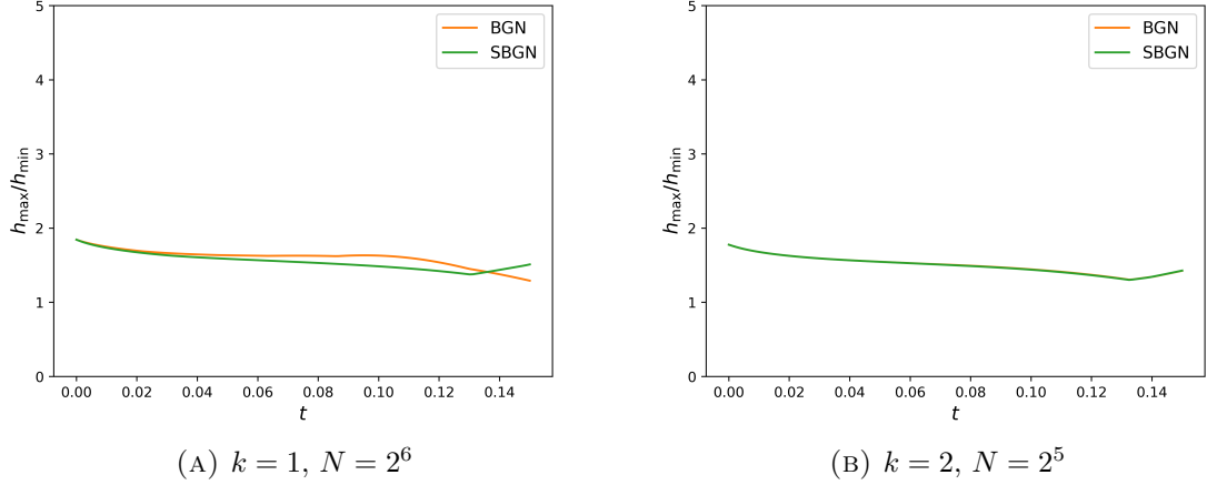
FIGURE 3. Mesh ratio h_{\max}/h_{\min} .
