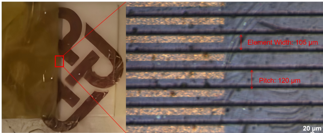
Fig. 2. Photograph of developed TUT array.
