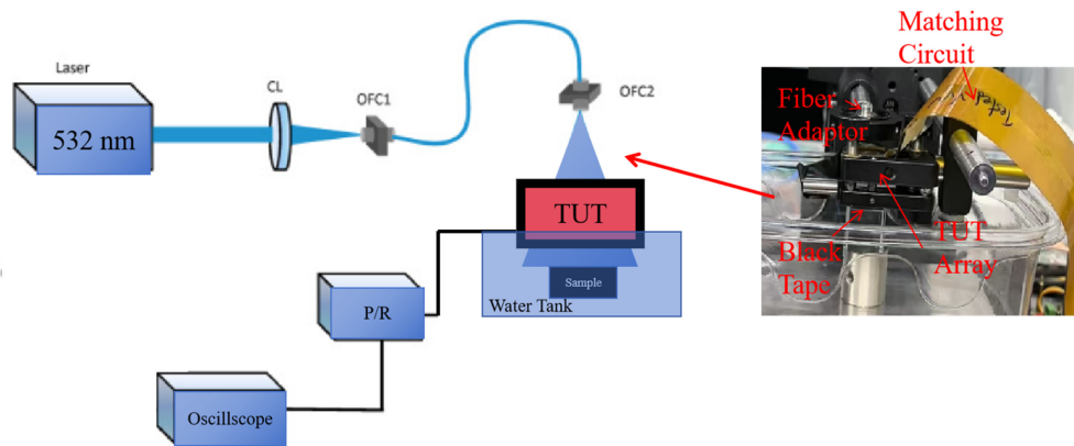
Fig. 1. Schematic of photoacoustic system based on TUT array. CL: Coupled lens; OFC: Optical fiber connector; P/R: Pulser/receiver.
