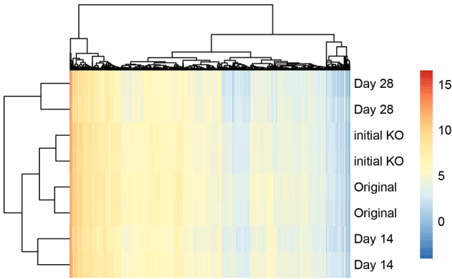
Figure 4. Heatmap of gene expression profiles for replicates of the original strain and ADE1 knockout strains at different cultivation times
