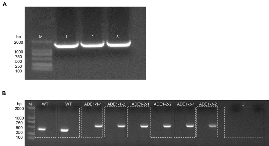
Figure 3. Gel electrophoresis from PCR of ADE1-URA3 fragment and Confirmation of the deleted loci of all samples in deletion lines
