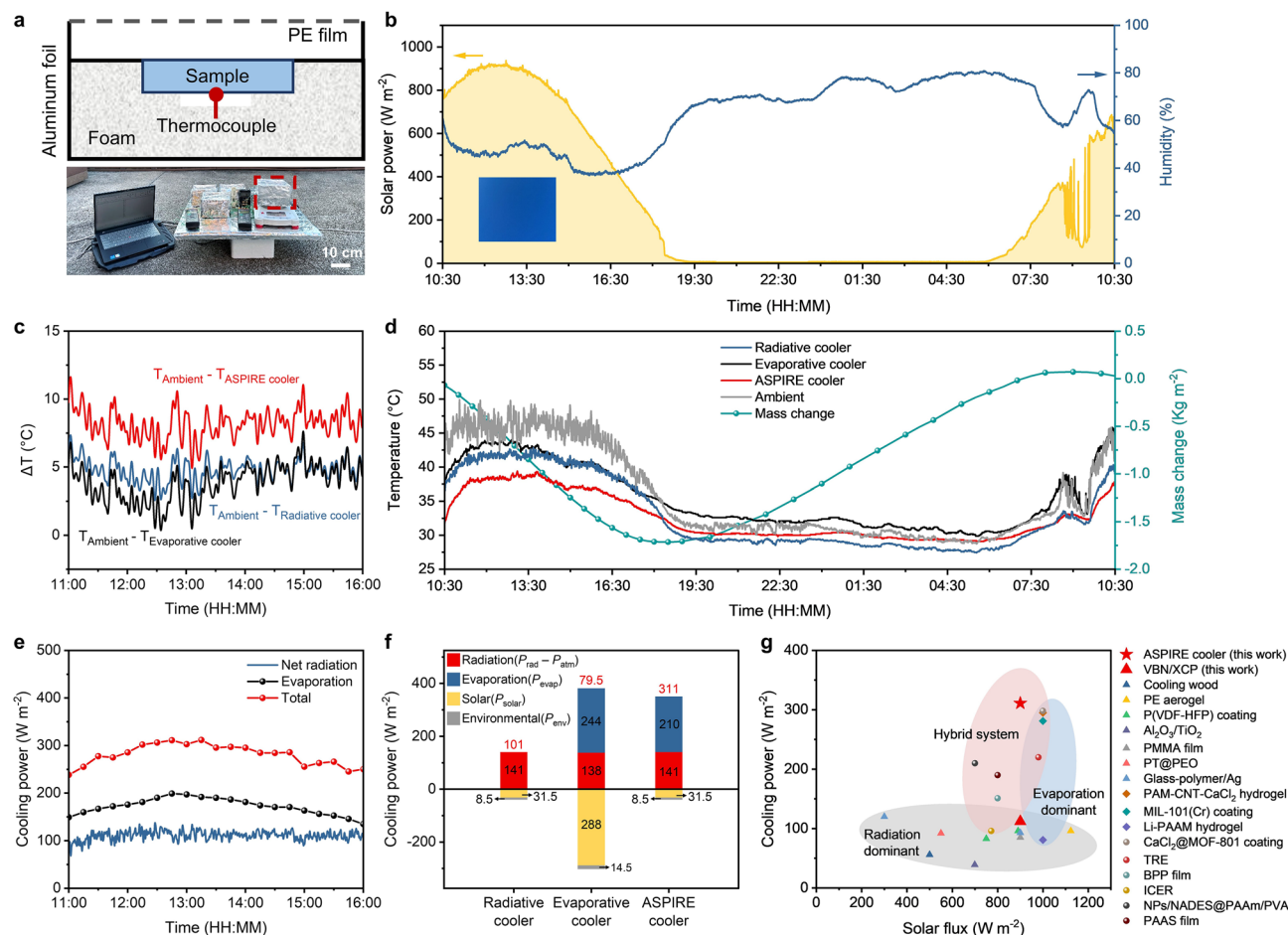
Fig. 5 Sub-ambient cooling performance and synergistic insulation-radiation-evaporation cooling mechanism of the ASPIRE cooler. a Schematic and photograph of the experimental setup used to measure the cooling performance in the outdoor test. The scale bar is 10 cm. b Solar power and RH during the test. Inset shows a photograph of the clear sky without any clouds. c Sub-ambient cooling temperature, \Delta T , during the test. d Temperatures of ASPIRE cooler, radiative cooler (i.e., VBN/XCP aerogel), evaporative cooler (i.e., V-PVA-LiCl hydrogel), and ambient, as well as the mass change of ASPIRE cooler during the test. e Contributions of evaporative and radiative-cooling powers to the total cooling power of the ASPIRE cooler. f Contributions of various cooling mechanisms to the total cooling powers of ASPIRE, radiative, and evaporative coolers. g Passive cooling power of ASPIRE cooler compared with others under different solar flux. Detailed data can be found in Table S2
