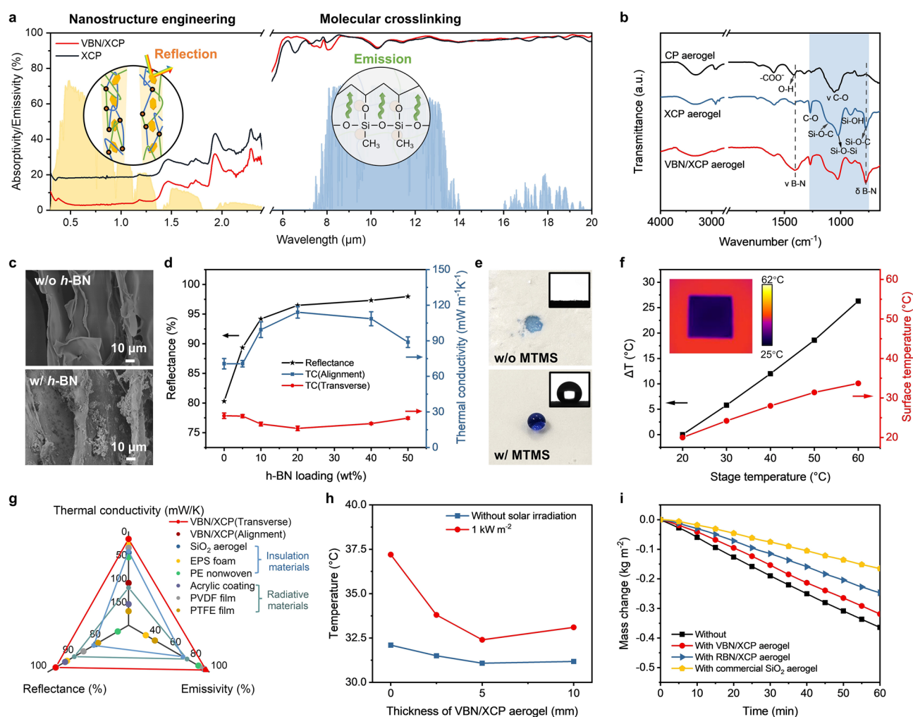
Fig. 4 Radiative, conductive, and vapor transport of the VBN/XCP aerogel. a Solar and LWIR absorption spectra of XCP and VBN/XCP aerogels. b FTIR spectra of CP, XCP, and VBN/XCP aerogel. c SEM images of XCP and VBN/XCP aerogels. d Solar-weighted reflectance and thermal conductivities of VBN/XCP aerogels with different h-BN loading. e Photographs of wetting states and water contact angles of VBN/CP aerogels with and without MTMS crosslinking. f Temperature differences between hot stage and VBN/XCP aerogel surface plotted against stage temperatures. Inset shows an IR image of the VBN/XCP aerogel on the hot stage with a temperature of 60 ^{\circ}\text{C} . g Comparison of key properties of VBN/XCP aerogel with other common radiative-cooling or insulation materials. h Temperatures of ASPIRE coolers with VBN/XCP aerogels of different thicknesses during evaporation at 40 ^{\circ}\text{C} and 40% RH. i Mass changes of V-PVA-LiCl hydrogel measured at 40 ^{\circ}\text{C} and 40% RH when covered without and with different aerogels
