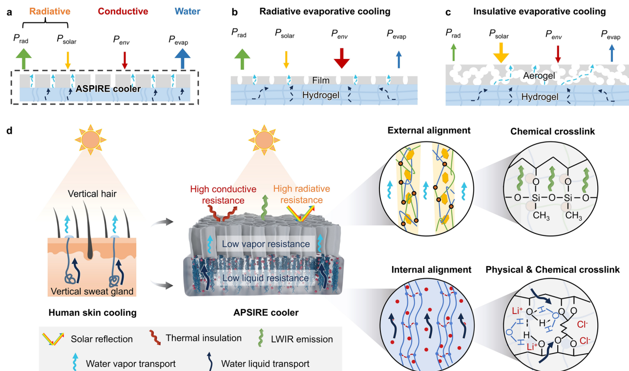
Fig. 1 Design principles of skin-inspired ASPIRE cooler. a Thermal balance of a hybrid insulative, radiative, and evaporative-cooling system. Existing bilayer design of b film-hydrogel and c aerogel-hydrogel architectures for evaporative cooling. d Schematic of the multiscale structural design of ASPIRE cooler inspired by human skin structure with the vertically aligned sweat glands and hair
