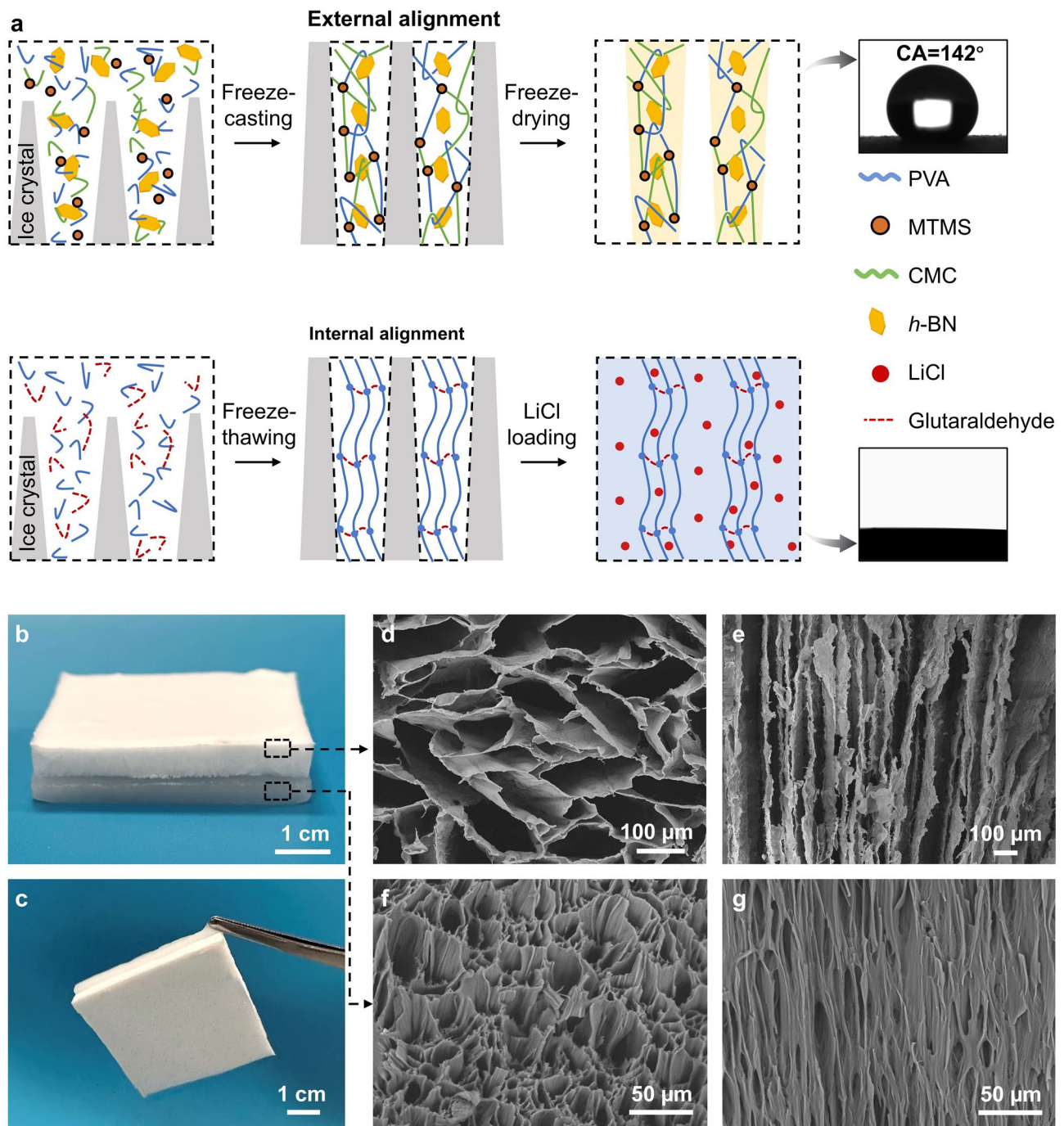
Fig. 2 Fabrication and structural characterization of ASPIRE cooler. a Schematics of the construction of internal and external alignments. Inset pictures show a water contact angle of 142° for the external alignment structure while a quick absorption of water in the internal alignment structure with no droplet remaining during the contact angle measurement. b Photograph of the ASPIRE cooler. c Photograph showing strong adhesion between internal and external alignment structures. d Top-view and e side-view SEM images of the external alignment structure. f Top-view and g side-view SEM images of internal alignment structure
