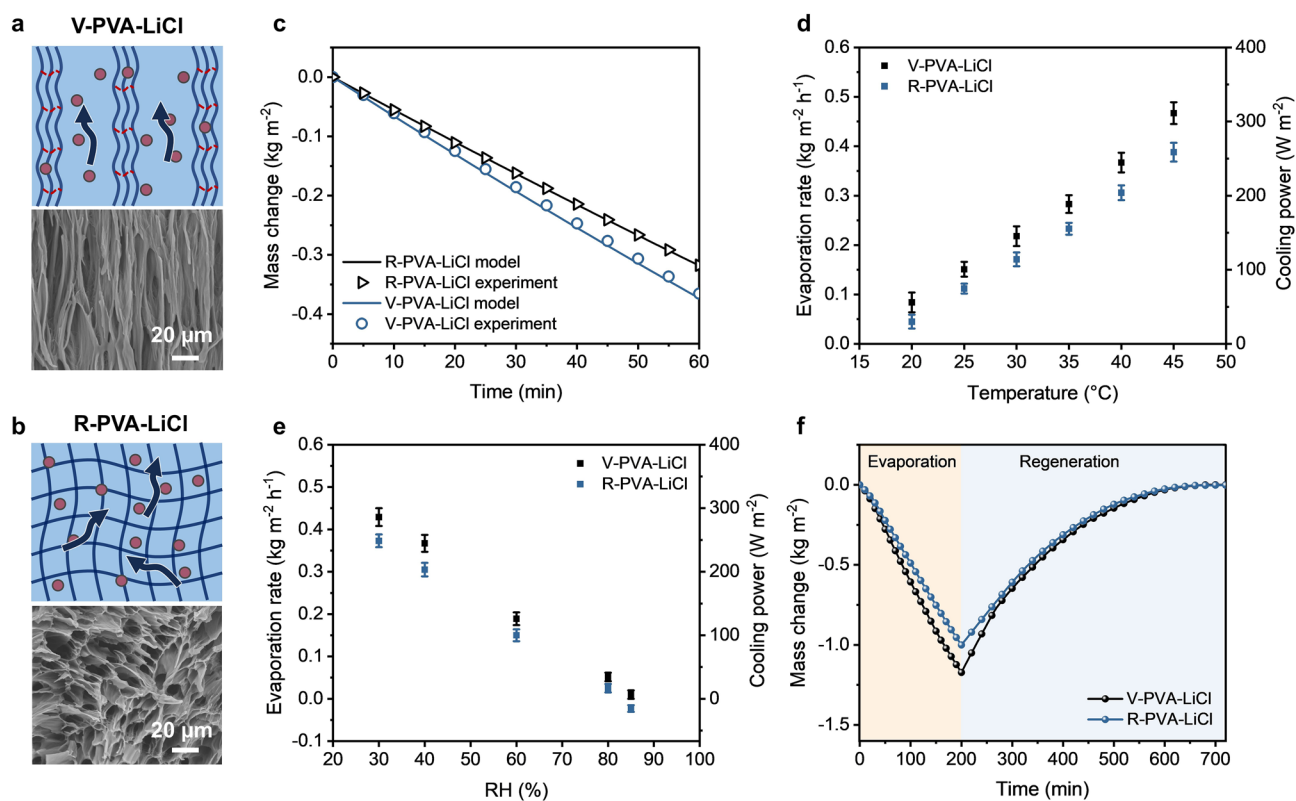
Fig. 3 Water evaporation and regeneration performance of V-PVA-LiCl hydrogel. a, b Schematics showing the mechanisms for better liquid and vapor transport in the V-PVA-LiCl hydrogel than the random one. c Model and experiment results of mass changes of V-PVA-LiCl and R-PVA-LiCl hydrogel measured at 40 °C and 40% RH. d Evaporation rates and calculated cooling powers of the two hydrogels for different RH at the same humidity of 40% RH. e Evaporation rates and calculated cooling powers of the two hydrogels for different RH at the same temperature of 40 °C. f Mass changes measured during consecutive evaporation (at 40 °C, 40% RH) and regeneration (at 25 °C, 80% RH) of V-PVA-LiCl and R-PVA-LiCl hydrogels
