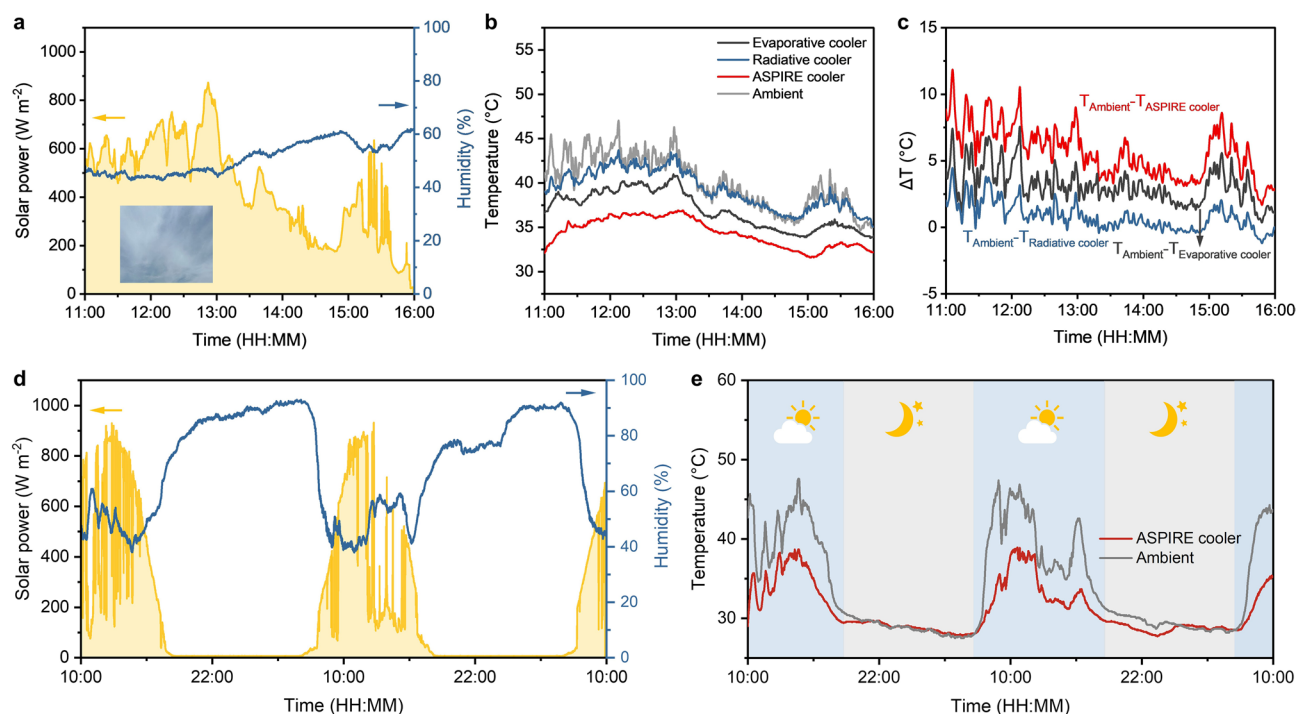
Fig. 6 All-weather, self-sustained multi-day cooling performance of ASPIRE cooler. a Solar intensity and RH of a cloudy day (Sep 4, 2023, in Hong Kong, China) when the outdoor cooling performance test was carried out. Inset shows a photograph of the cloudy sky taken during the test. b Temperatures and c sub-ambient cooling temperatures ( \Delta T ) of the three coolers. d Solar intensity and RH during the continuous test for 48 h from 19 to 21 September 2023, in Hong Kong, China. e Temperatures variations of the ASPIRE cooler and ambient during the continuous 48-h test
