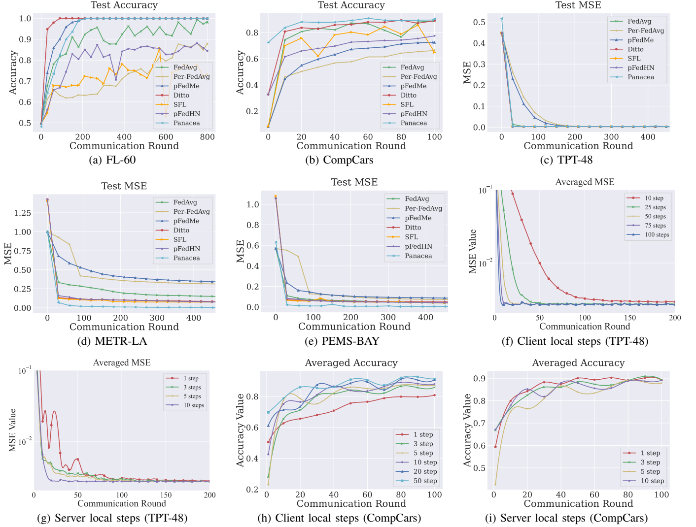
Fig. 3: (a)-(e) compare convergence speed and final performance, and (f)-(i) compare final performance of Panacea with various hyperparameter settings.
