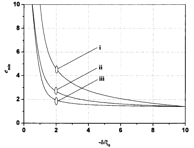
FIG. 3. Minimum switching field e_{\min} as a function of surface parameter for different thicknesses. The switching field is a pulsed Gaussian field with pulse width \sigma = 1000 . In the curves, the thicknesses are (i) L = 2.0\xi_0 , (ii) L = 5.0\xi_0 , and (iii) L = 10.0\xi_0 .
