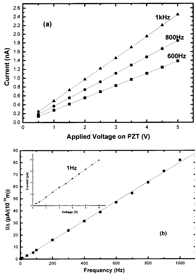
FIG. 3. (1) The current measured by a lock-in amplifier at different frequencies vs displacement in a PZT standard (the displacement in PZT= 4.91 \text{ Å} \times Applied Voltage) cure. (b) The calibration curve of the bimorph sensor. The inserted graph is the calibration curve of 1 Hz with 30 s time constant of the lock-in amplifier. Open circles are the experimental data and solid line is a linear fitting curve.
