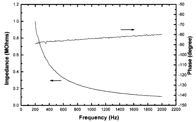
FIG. 9. The electric impedance and phase of No. 3 head measured from the bimorph when the probe head was in contact with a PZT sample on platform shown in Fig. 4(b). There is no resonance at frequencies below 2 kHz and the other sensor heads are similar to No. 3. When operating at low frequencies, a long time constant of a lock-in amplifier is preferred.
