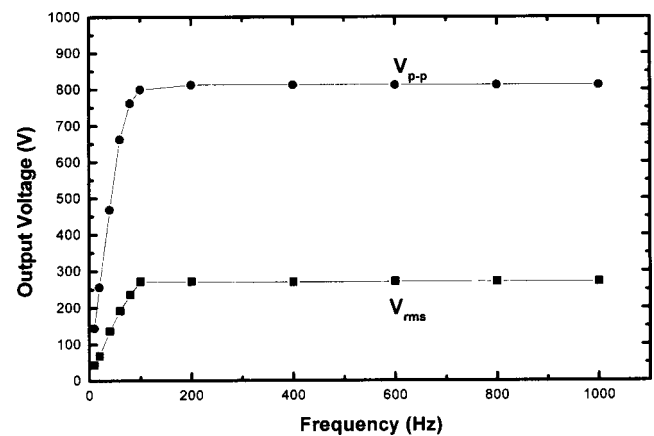
FIG. 10. The output voltage as a function of frequency when a commercial P(VDF-TrFE) (80/20 mol %, 25 pC/N, 30 \mu\text{m} ) copolymer film was used to calibrate the setup. V_{p-p} was the peak voltage and V_{rms} was the root of mean square voltage.
