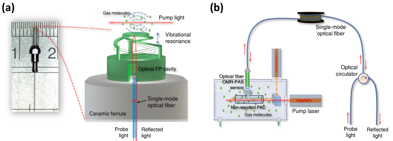
Fig. 1. Schematics of an optical fiber OMR-PAS gas sensor and its application in a PAS trace-gas detection microsystem. (a) Schematic design of an optical fiber OMR-PAS gas sensor based on a ferrule-top PSS-OMR. (b) Schematic of a non-resonant PAC enhanced optical fiber PAS trace-gas detection microsystem.
