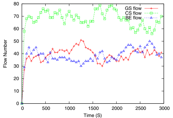
Fig. 5. Flows generated in simulations
