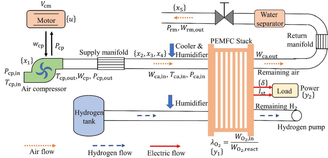
Fig. 5. PEMFC gas management subsystems [31].
