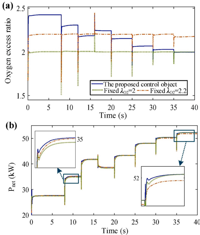
Fig. 6. Effects of different control strategies on OER and output net power changes[21].
