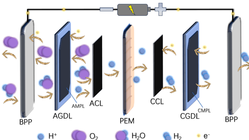
Fig. 2. Schematic and operational fundamentals of PEMWE.
