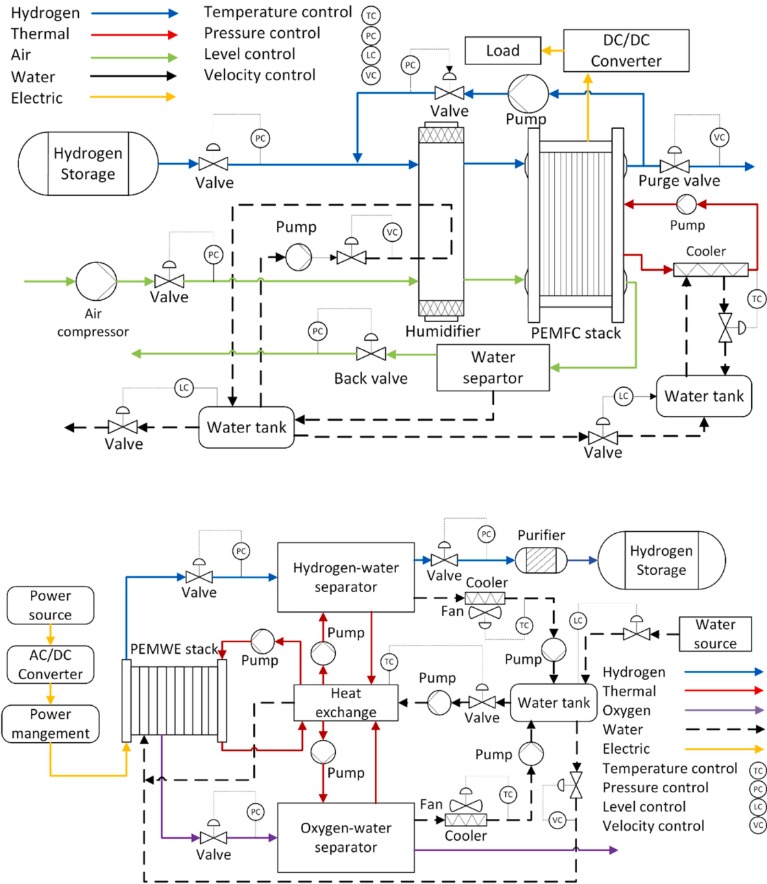
Fig. 4. Combined control systems of PEMFC (top) and PEMWE (down) stacks.
