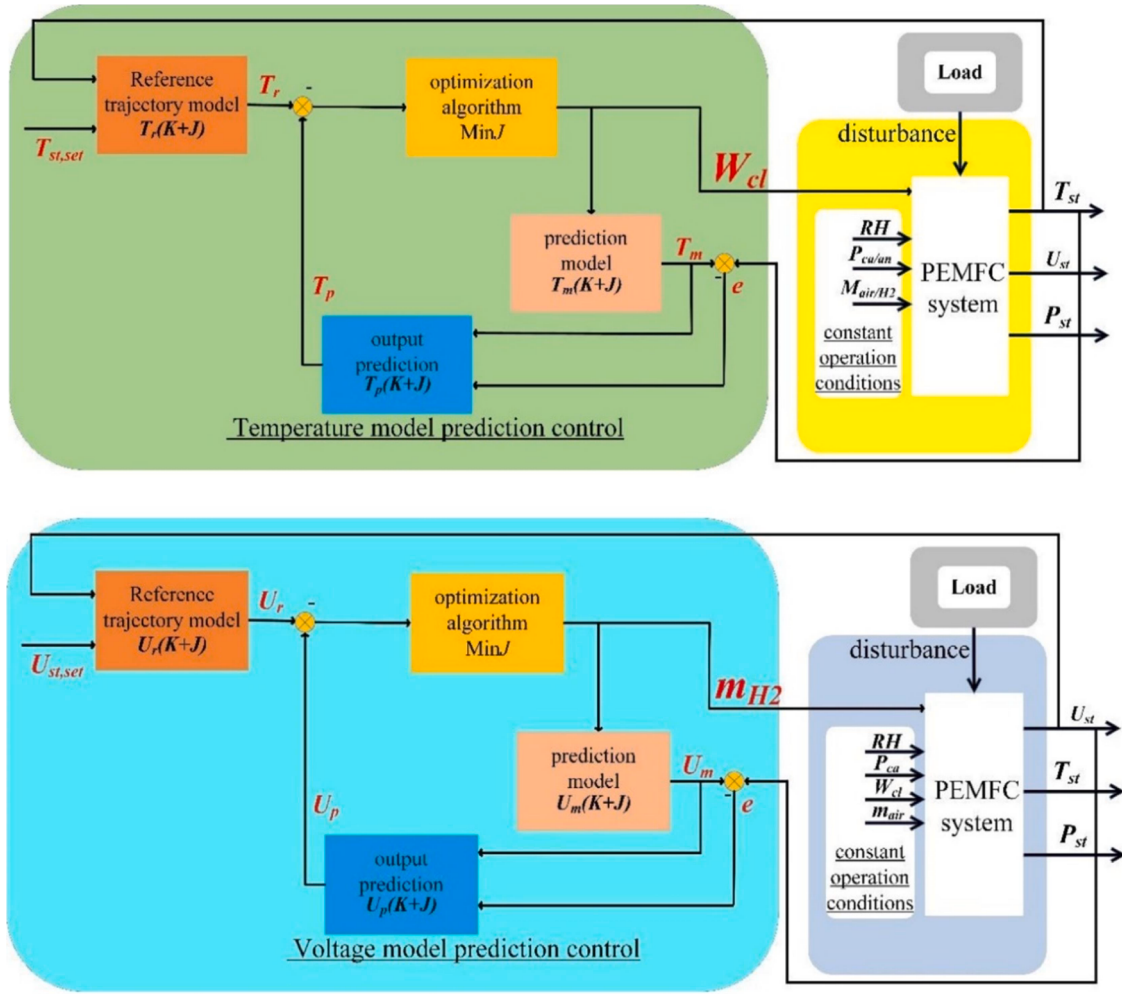
Fig. 15. MPC system for temperature (top) and voltage (down) control [83].
