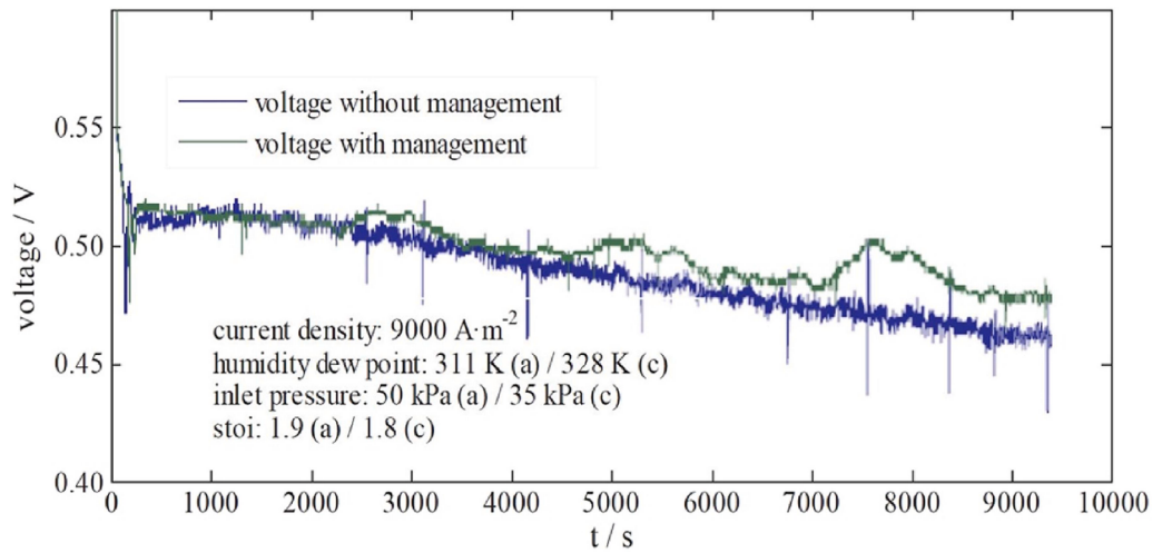
Fig. 8. Voltage changes before and after the application of water management system in PEMFC [54].
