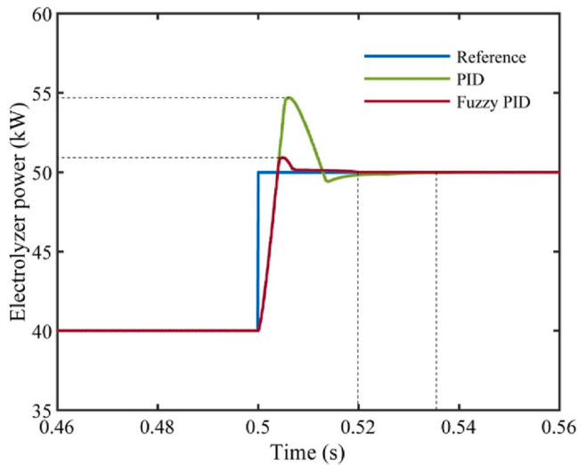
Fig. 9. Effects of different control strategies on input power changes in PEMWE [60].
