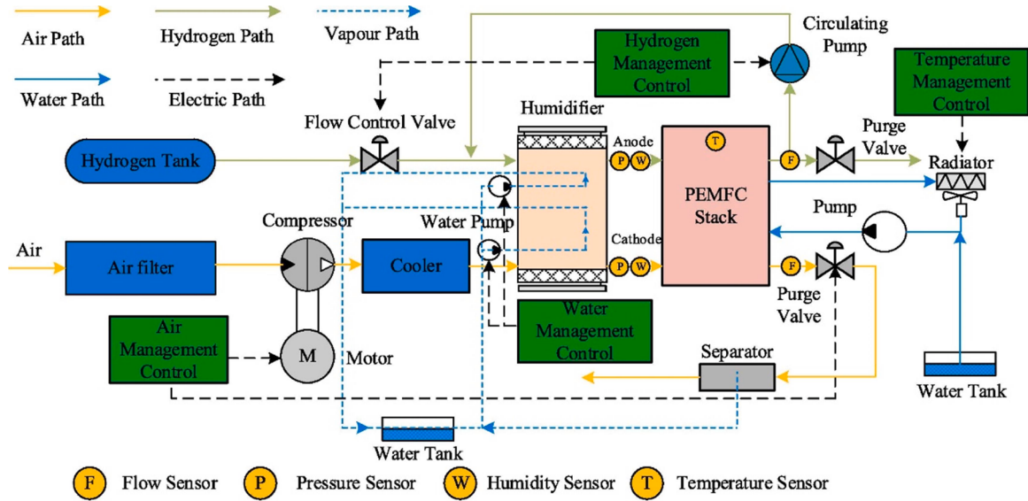
Fig. 10. A promising PEMFC subsystem design strategy [70].
