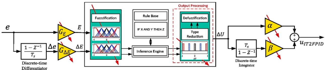
Fig. 13. FLC control system design [80].
