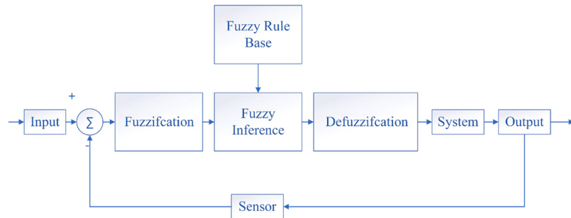
Fig. 12. Typical FLC structure.
