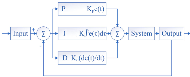
Fig. 11. Fundamental PID structure.
