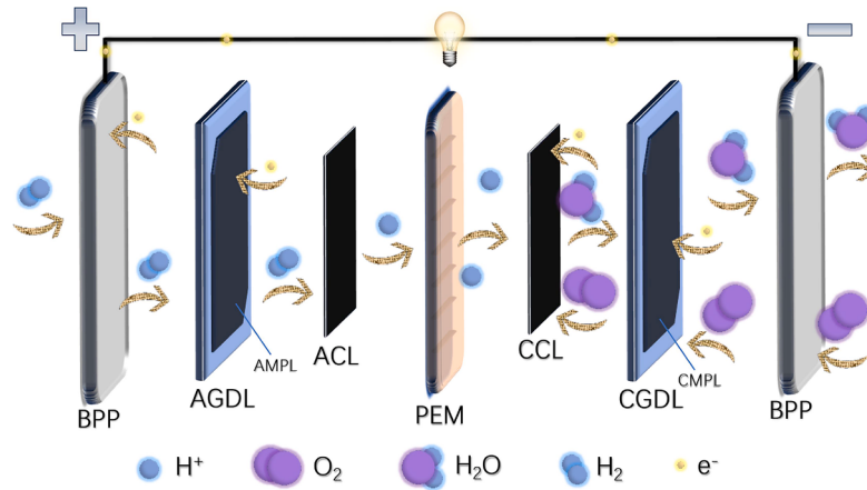
Fig. 1. Schematic and operational fundamentals of PEMFC.
