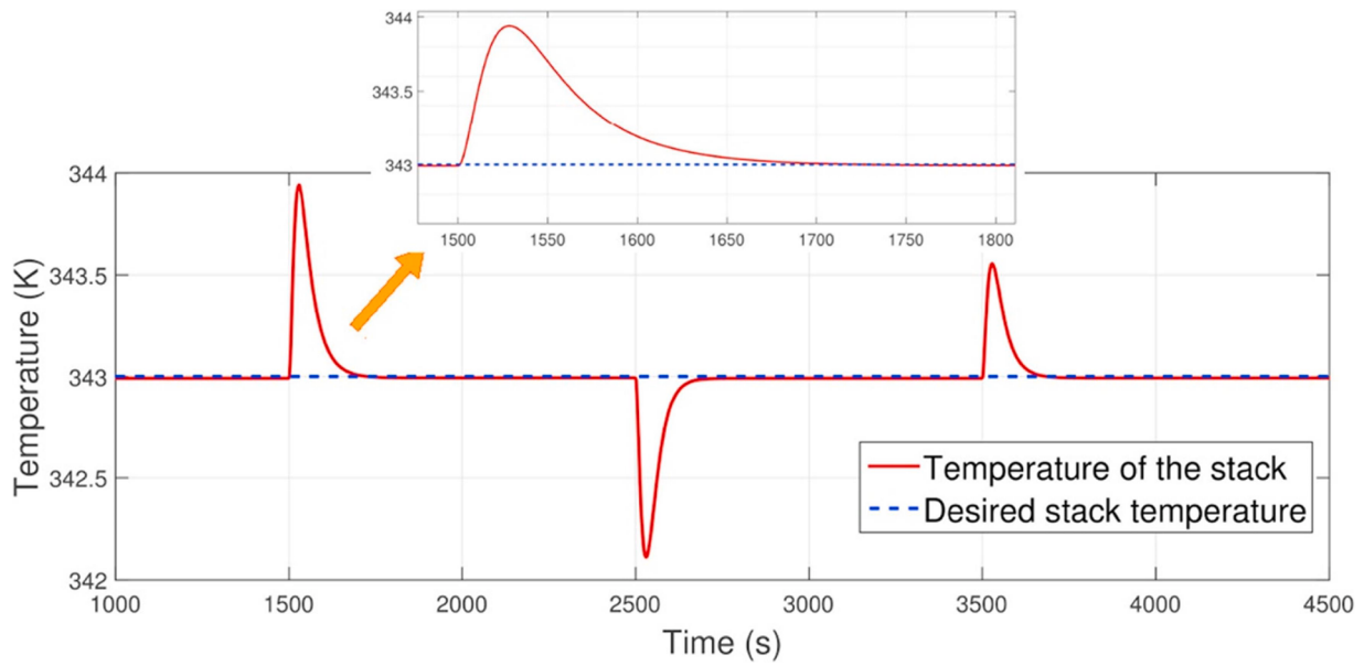
Fig. 7. Temperature changes before and after control system application in PEMFC [42].
