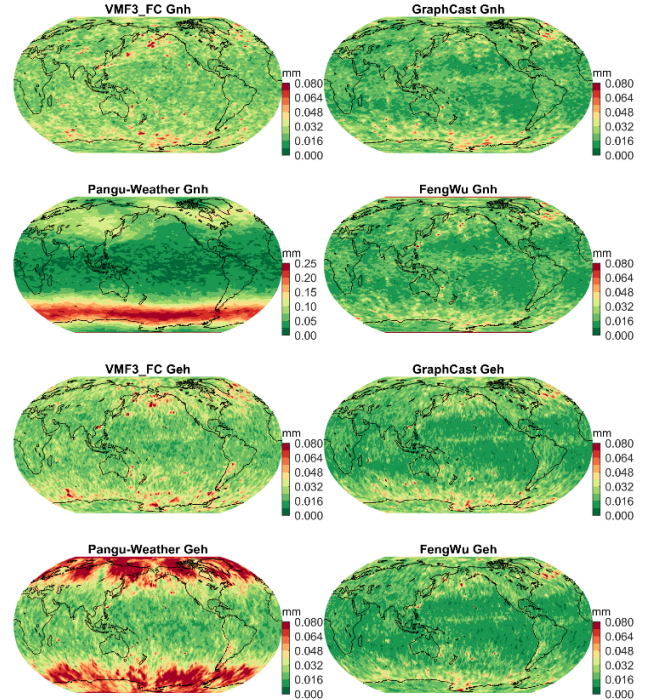
Fig. A11. Comparison of VMF3_FC, Pangu-Weather, GraphCast, and FengWu hydrostatic gradient accuracy. Note the different color bar scales of the panels.
