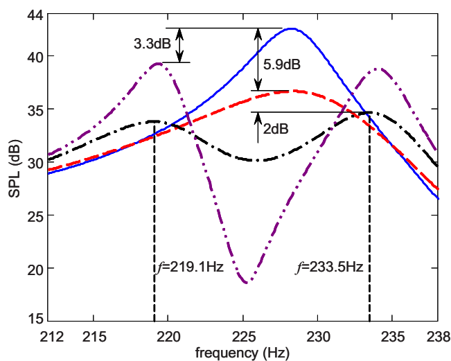
FIG. 10. (Color online) Predicted SPLs at (0.816, 0.07, 1.028) m: — without resonator; - - with resonator, R_i=19.94 mks Rayls from Fahy and Schofield's resonance-control model; — with resonator, R_i=1.1 mks Rayls from Fahy and Schofield's band-control model; and ··· with resonator, R_i=5.93 mks Rayls from current model.
