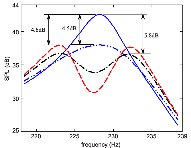
FIG. 4. (Color online) Predicted SPL curves at (0.816, 0.07, 1.028) m: —without resonator; ---with a damped resonator, R_i=3.82 mks Rayls; - - with an empty-neck resonator, R_i=2.25 mks Rayls; and — with a damped resonator, R_i=9.62 mks Rayls.
