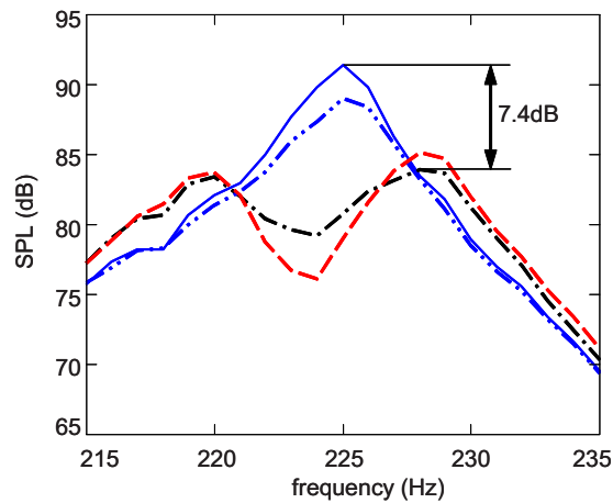
FIG. 5. (Color online) Measured SPL curves at (0.816, 0.07, 1.028) m: — without resonator; — with a damped resonator, R_i=3.59 mks Rayls; -- with an empty-neck resonator, R_i=2.25 mks Rayls; and -·- with a damped resonator, R_i=9.62 mks Rayls.
