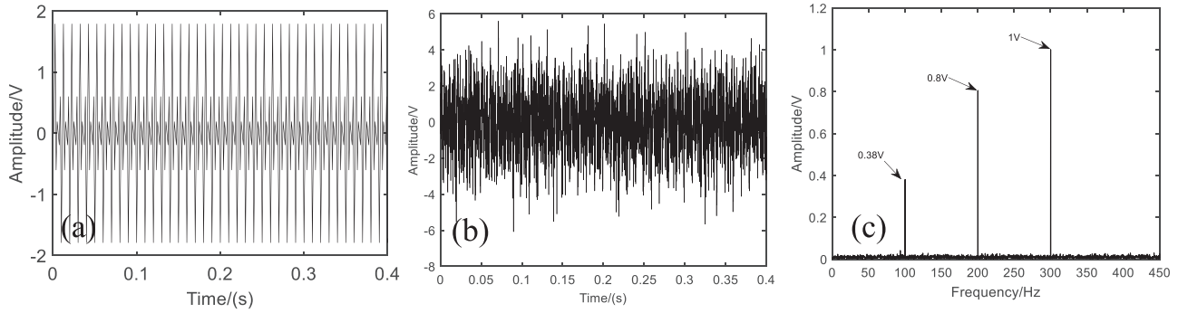
FIG. 3. The simulated input noise signal r(t) , (a) the pure tone signal, (b) the noise added signal (SNR=-3dB), and (c) the frequency spectrum.
