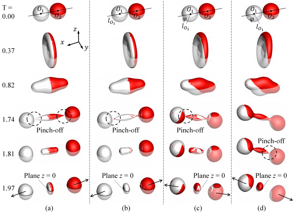
FIG. 4. Evolution of droplet deformation upon a head-on collision of (a) two nonspinning droplets and of a spinning droplet O_1 and a nonspinning droplet O_2 with varying azimuthal angle of droplet O_1 (b) \phi = 0 , (c) \phi = \pi/4 , and (d) \phi = \pi/2 , at We = 61.4 , Oh = 0.028 , and \omega_0 = 3 .
