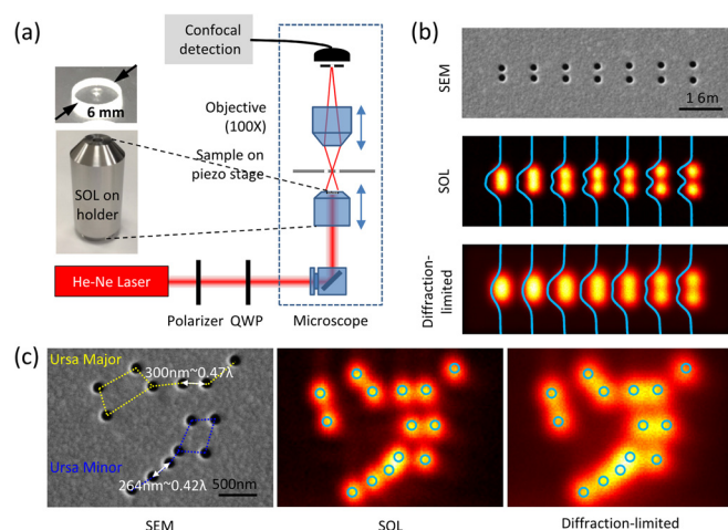
FIG. 3. (a) Schematics of the experimental setup for the imaging with the superoscillatory hotspot and confocal detection. The insets show the 1.2 mm-diameter SOL in the laser diced quartz substrate with a 6 mm diameter (top) and the self-manufactured holder with an open aperture to fit the SOL (bottom). (b) SEM image, superoscillatory (with SOL), and diffraction-limited (with a normal objective of NA = 0.95 ) imaging of hole pair arrays with varying center-to-center distance from 210 nm to 390 nm with a step size of 30 nm. Hole diameter: 160 nm. (c) SEM image, superoscillatory, and diffraction-limited imaging of a complex image (Ursa Major in yellow and Ursa Minor in blue) with varying hole center-to-center distance. Hole diameter: 160 nm.
