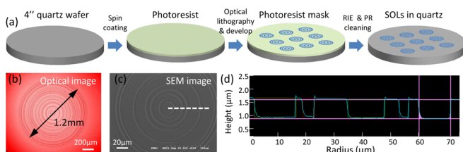
FIG. 1. (a) Fabrication procedures of the quartz superoscillatory lens (SOL), including spin coating, lithography and development of photoresist, reactive ion etching, and photoresist cleaning. (b) Optical image of an SOL with a diameter of 2R = 1.2 \text{ mm} . (c) SEM image of the central part of the SOL. (d) Profile of the lens measured along the white dashed line in (c) shows an etching depth of 710 \text{ nm} \pm 18 \text{ nm} corresponding to a phase delay of (1.1 \pm 0.03)\pi at a wavelength of 633 \text{ nm} .
