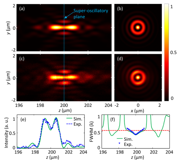
FIG. 2. (a) Simulated longitudinal cross section of the superoscillatory hotspot near an axial distance of 200 \mu\text{m} . (b) Simulated intensity profile in the transverse plane. (c) Experimentally measured longitudinal cross section of the superoscillatory hotspot in the same area of interest. (d) Experimental intensity profile in the transverse plane. (e) Comparison of the axial intensity of the hotspot between the simulation (green curve) and experiment (blue dashed curve). (f) Comparison of the spot size between the simulation (green curve) and experiment (blue down triangle). The red dashed line shows the Abbe diffraction limit defined by \lambda/(2\text{NA}) = 0.53\lambda .
