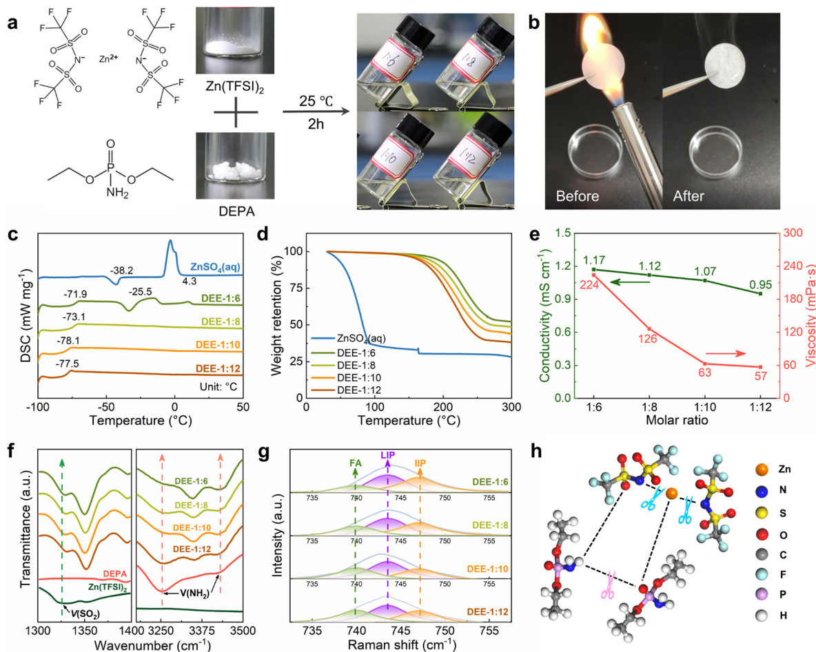
Fig. 1 Physicochemical properties and spectral analysis of DEEs. (a) Preparation strategy of DEEs based on \text{Zn}(\text{TFSI})_2 and DEPA. (b) Flammability test of separator soaked by DEE under open flame lighter. (c) DSC curves of \text{ZnSO}_4 aqueous electrolyte and DEEs with different \text{Zn}(\text{TFSI})_2 : DEPA molar ratios from -100^\circ\text{C} to 50^\circ\text{C} . (d) TGA results of \text{ZnSO}_4 aqueous electrolyte and different DEEs. (e) Ionic conductivity and viscosity of different DEEs. (f) FTIR spectra: \nu(\text{SO}_2) and \nu(\text{NH}_2) . (g) Fitted Raman spectra of DEEs with different molar ratios. (h) Illustration of the interaction among \text{Zn}^{2+} , \text{TFSI}^- and DEPA in DEEs.
